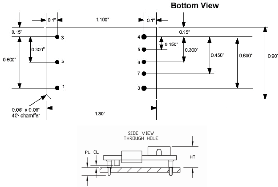
SSQE48T Pinout (Through-hole)
