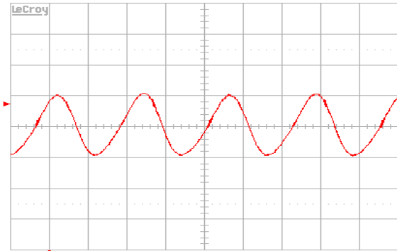
Figure 10. Output voltage ripple (10 mV/div.) at full rated load current into a resistive load with C_o = 10 \mu\text{F} tantalum + 1 \mu\text{F} ceramic and V_{in} = 48 \text{ V} . Time scale: 1 \mu\text{s}/\text{div} .
