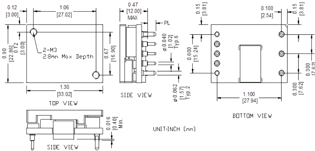
SSQE48T Pinout (Through-hole)
