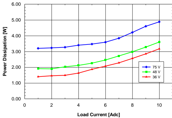
Figure 4. Power dissipation vs. load current and input voltage for SSQE48T10033 converter mounted vertically with air flowing from pin 1 to pin 3 at a rate of 300 LFM (1.5 m/s) and T_a = 25^\circ C .
