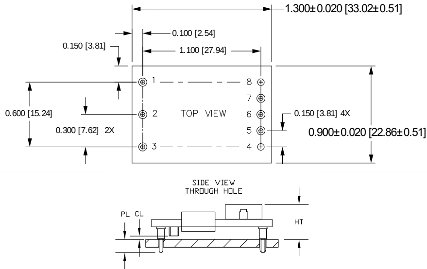
SSQE48T Pinout (Through-hole)
