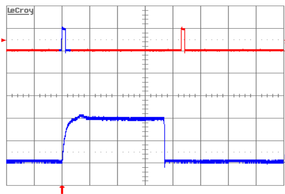
Figure 15. Load current (top trace, 20 A/div., 50 ms/div.) into a 10 m \Omega short circuit during restart, at V_{in} = 48 V. Bottom trace (10 A/div., 2 ms/div.) is an expansion of the on-time portion of the top trace
