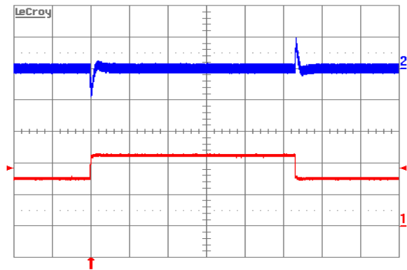
Figure 9. Output voltage response to load current step-change (7.5 A–10.25 A–7.5 A) at V_{\text{in}} = 48\text{ V} . Top trace: output voltage (100 mV/div.). Bottom trace: load current (5 A/div.). Current slew rate: 5 A/ \mu\text{s} . C_o = 470\mu\text{F} POS + 1 \mu\text{F} ceramic. Time scale: 0.2 ms/div.
