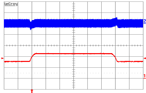
Figure 8. Output voltage response to load current step-change (7.5 A–10.25 A–7.5 A) at V_{\text{in}} = 48\text{ V} . Top trace: output voltage (100 mV/div.). Bottom trace: load current (5 A/div.). Current slew rate: 0.1 A/ \mu\text{s} . C_o = 1\mu\text{F} ceramic + 10 \mu\text{F} tantalum. Time scale: 0.2 ms/div.
