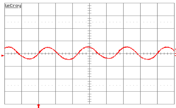
Figure 13. Input reflected ripple-current, i_c (200 mV/div.), measured at input terminals at full rated load current and V_{in} = 48 V. Refer to Figure 11 for test setup. Time scale: 1 \mu s/div.
