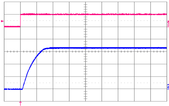
Figure 7. Turn-on transient at full rated load current (resistive) plus 20,000 \mu\text{F} at V_{\text{in}} = 48\text{ V} , triggered via ON/OFF pin. Top trace: ON/OFF signal (5 V/div.). Bottom trace: Output voltage (1 V/div.). Time scale: 5 ms/div.
