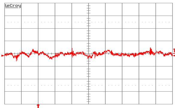
Figure 12. Input reflected-ripple current, is (10 mV/div.), measured through 10 \mu H at the source at full rated load current and V_{in} = 48 V. Refer to Figure 11 for test setup. Time scale: 1 \mu s/div.
