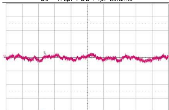
Figure 14. Input reflected-ripple current, is (10 mA/div.), measured through 10 uH at the source at full rated load current and Vin = 48 V. Refer to Fig. J for test setup. Time scale: 1us/div.
