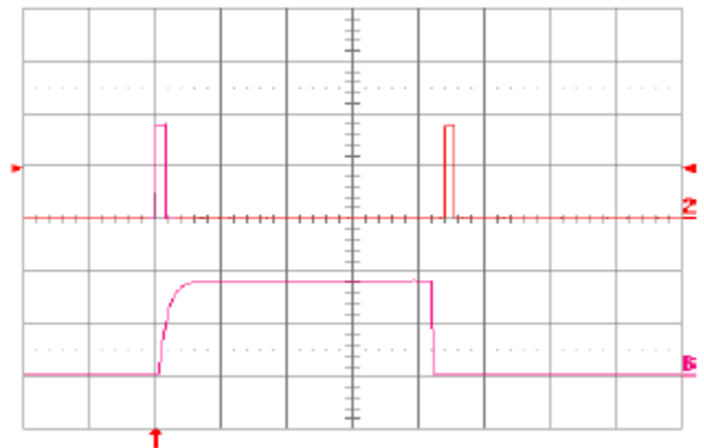
Fig. 2.5V.16: Load current (top trace, 20 \text{ A}/\text{div} ., 50 \text{ ms}/\text{div} .) into a 10 \text{ m}\Omega short circuit during restart, at V_{in} = 48 \text{ V} . Bottom trace ( 20 \text{ A}/\text{div} ., 2 \text{ ms}/\text{div} .) is an expansion of the on-time portion of the top trace.
