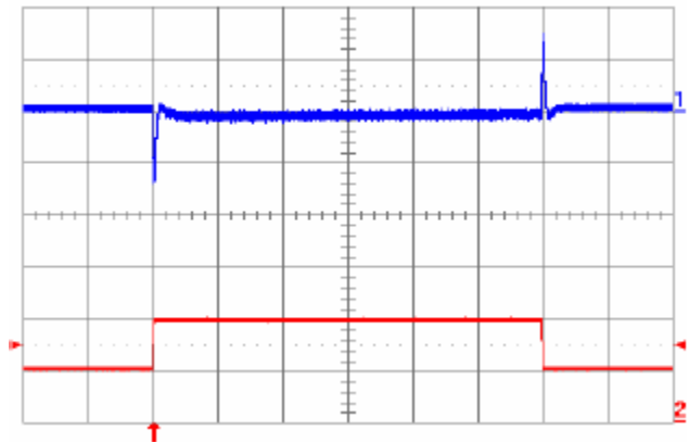
Fig. 3.3V.10: Output voltage response to load current step-change (10 A – 20 A – 10 A) at V_{in} = 48 V. Top trace: output voltage (100 mV/div.). Bottom trace: load current (10 A/div.). Current slew rate: 5 A/ \mu s. C_o = 470 \mu F POS + 1 \mu F ceramic. Time scale: 0.2 ms/div.
