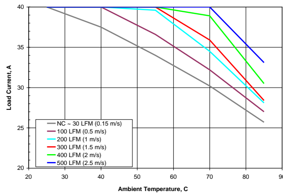
Figure 1. Available load current vs. ambient air temperature and airflow rates for SQE48T40018 converter mounted vertically with air flowing from pin 3 to pin 1, MOSFET temperature \leq 120\text{ }^\circ\text{C} , V_{in} = 48\text{ V} . Note: NC – Natural convection
