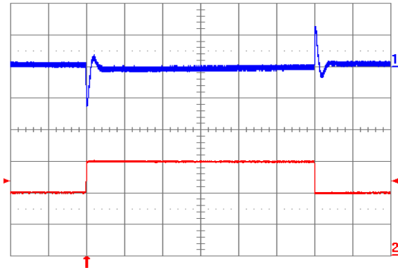
Fig. 10: Output voltage response to load current step-change (10 A - 15 A - 10 A) at V_{in} = 48\text{ V} . Top trace: output voltage (100 mV/div.). Bottom trace: load current (5 A/div.). Current slew rate: 5 A/ \mu\text{s} . C_o = 470\ \mu\text{F} POS + 1 \mu\text{F} ceramic. Time scale: 0.2 ms/div.
