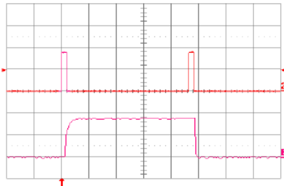
Fig. 1.5V.16: Load current (top trace, 20 A/div., 50 ms/div.) into a 10 mΩ short circuit during restart, at V_{in} = 48\text{ V} . Bottom trace (20 A/div., 2 ms/div.) is an expansion of the on-time portion of the top trace.
