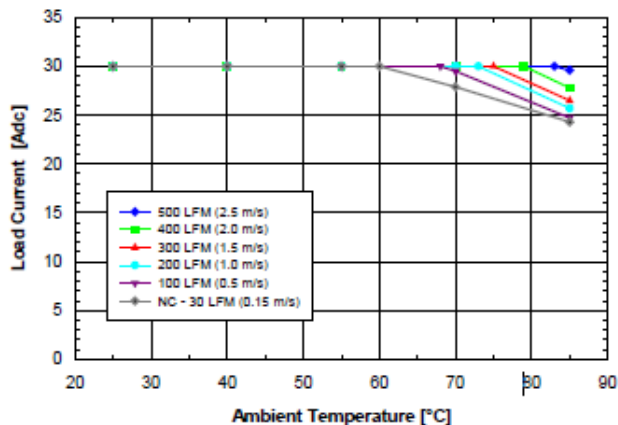
Fig. 1.2V.1: Available load current vs. ambient air temperature and airflow rates for SQE48T30012 converter mounted vertically with air flowing from pin 3 to pin 1, MOSFET temperature \leq 120^\circ\text{C} , V_{in} = 48\text{ V} .
