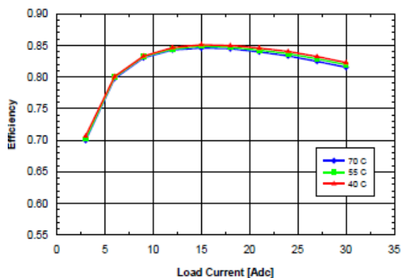
Fig. 1.2V.4: Efficiency vs. load current and ambient temperature for SQE48T30012 converter mounted vertically with V_{in} = 48\text{ V} and air flowing from pin 3 to pin 1 at a rate of 200 LFM (1.0 m/s).
