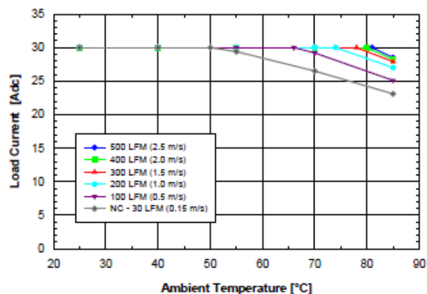
Fig. 1.2V.2: Available load current vs. ambient air temperature and airflow rates for SQE48T30012 converter mounted horizontally with air flowing from pin 3 to pin 1, MOSFET temperature \leq 120^\circ\text{C} , V_{in} = 48\text{ V} .
