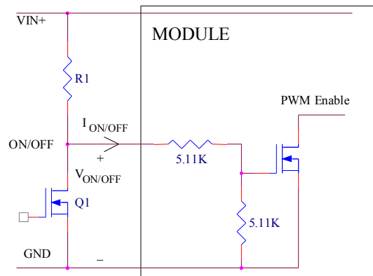
Remote On/Off Implementation using ON/OFF
