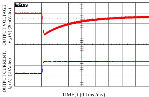
Transient Response to Dynamic Load Change from 50% to 100%. V_o=1.8V , T_a=25^\circ C , V_{in}=12V , C_{ext}=5x47\mu F+8x330\mu F polymer, C_{Tune}=47nF , R_{Tune}=220ohms
