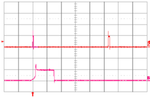
Fig. 1.8V.18: Load current (top trace, 20\text{A}/\text{div} ., 20\text{ms}/\text{div} .) into a 10\text{m}\Omega short circuit during restart, at V_{in} = 48\text{V} . Bottom trace ( 20\text{A}/\text{div} ., 1\text{ms}/\text{div} .) is an expansion of the on-time portion of the top trace.
