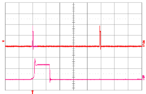
Fig. 5.0V.18: Load current (top trace, 10A/div., 20 ms/div.) into a 10 m \Omega short circuit during restart, at V_{in} = 48\text{V} . Bottom trace (10A/div., 1ms/div.) is an expansion of the on-time portion of the top trace.
