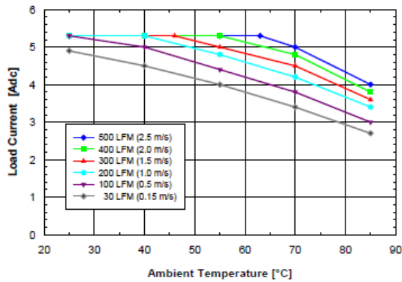
Figure 8.0V.1 Available load current vs. ambient air temperature and airflow rates for SQ48T05080 converter with D height pins mounted vertically with V_{in} = 48V , air flowing from pin 3 to pin 1, and maximum FET temperature \leq 120^{\circ}C .
