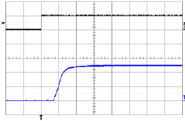
Fig. 5.0V.9: Turn-on transient at full rated load current (resistive) with no output capacitor at V_{in} = 48V , triggered via ON/OFF pin. Top trace: ON/OFF signal (5V/div.). Bottom trace: output voltage (2V/div.). Time scale: 2ms/div.
