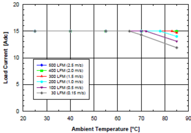
Figure 1.8V.1 Available load current vs. ambient air temperature and airflow rates for SQ48T15018 converter with D height pins mounted vertically with V_{in} = 48V , air flowing from pin 3 to pin 1, and maximum FET temperature \leq 120^{\circ}C .
