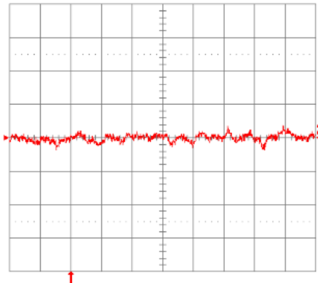
Fig. 2.0V.16: Input reflected ripple current, i_s (10 mA/div.), measured through 10\mu\text{H} at the source at full rated full rated load current and V_{in} = 48\text{V} . Refer to Fig. 2.0V.14 for test setup. Time scale: 1\mu\text{s}/\text{div} .
