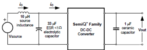
Fig. 2.5V.14: Test Setup for measuring input reflected ripple currents, i_c and i_s
