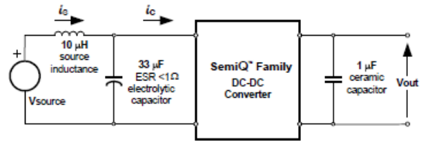
Fig. 3.3V.14: Test Setup for measuring input reflected ripple currents, i_c and i_s
