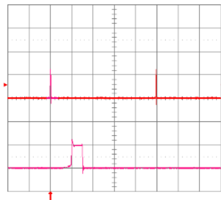
Fig. 2.5V.18: Load current (top trace, 20A/div., 20 ms/div.) into a 10\text{m}\Omega short circuit during restart, at V_{in} = 48\text{V} . Bottom trace (20A/div., 1ms/div.) is an expansion of the on-time portion of the top trace.
