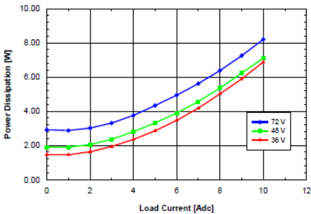
Fig. 5.0V.7: Power dissipation vs. load current and input voltage for SQ48T/S10050 converter mounted vertically with air flowing from pin 3 to pin 1 at a rate of 300 LFM (1.5 m/s) and T_a = 25^\circ\text{C} .
