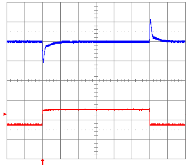
Fig. 1.5V.12: Output voltage response to load current step-change (3.75 A – 7.5 A – 3.75 A) at V_{in} = 48V . Top trace: output voltage (100 mV/div.). Bottom trace: load current (5A/div.). Current slew rate: 5 A/ \mu s . C_o = 450\mu F tantalum + 1 \mu F ceramic. Time scale: 0.2 ms/div.
