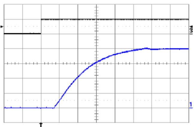
Fig. 8.0V.8: Turn-on transient at full rated load current (resistive) plus 2,200 µF at V_{in} = 48\text{V} , triggered via ON/OFF pin. Top trace: ON/OFF signal (5V/div.). Bottom trace: output voltage (2V/div.). Time scale: 2ms/div.
