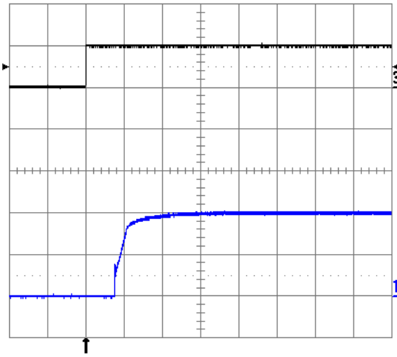
Fig. 2.0V.9: Turn-on transient at full rated load current (resistive) with no output capacitor at V_{in} = 48V , triggered via ON/OFF pin. Top trace: ON/OFF signal (5V/div.). Bottom trace: output voltage (1V/div.). Time scale: 2ms/div.
