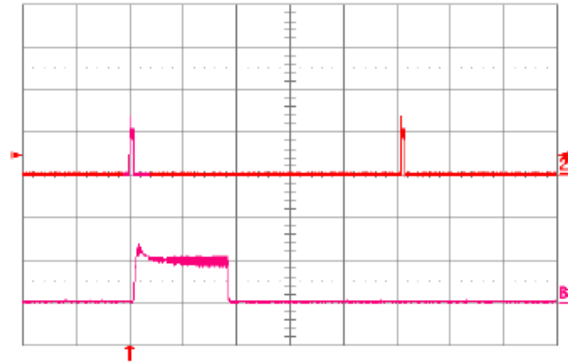
Fig. 12V.16: Load current (top trace, 5A/div., 20 ms/div.) into a 10 m \Omega short circuit during restart, at V_{in} = 48V . Bottom trace (5A/div., 1ms/div.) is an expansion of the on-time portion of the top trace.
