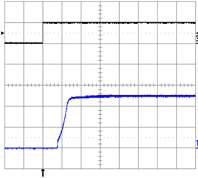
Fig. 2.5V.9: Turn-on transient at full rated load current (resistive) with no output capacitor at V_{in} = 48V , triggered via ON/OFF pin. Top trace: ON/OFF signal (5V/div.). Bottom trace: output voltage (1V/div.). Time scale: 2ms/div.
