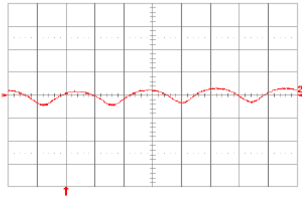
Fig. 1.0V.15: Input reflected ripple current, i_c (100 mA/div.), measured at input terminals at full rated load current and V_{in} = 48\text{V} . Refer to Fig. 1.0V.14 for test setup. Time scale: 1\mu\text{s}/\text{div} .
