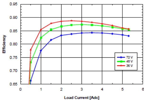
Fig. 8.0V.3: Efficiency vs. load current and input voltage for SQ48T/S05080 converter mounted vertically with air flowing from pin 3 to pin 1 at a rate of 300LFM (1.5 m/s) and T_a = 25^{\circ}C .
