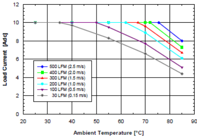
Figure 5.0V.1 Available load current vs. ambient air temperature and airflow rates for SQ48T10050 converter with D height pins mounted vertically with V_{in} = 48V , air flowing from pin 3 to pin 1, and maximum FET temperature \leq 120^{\circ}C .
