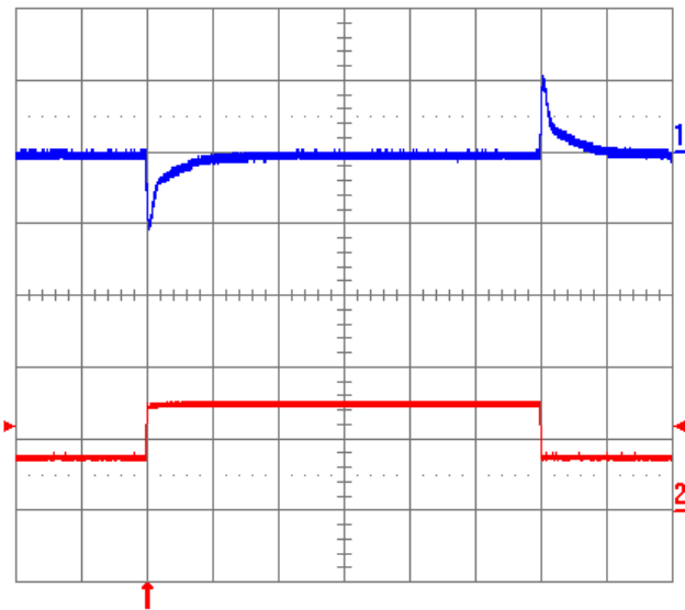
Fig. 1.8V.12: Output voltage response to load current step-change (3.75 A - 7.5 A - 3.75 A) at V_{in} = 48V . Top trace: output voltage (100 mV/div.). Bottom trace: load current (5A/div.). Current slew rate: 5 A/ \mu s . C_o = 450\mu F tantalum + 1 \mu F ceramic. Time scale: 0.2 ms/div.
