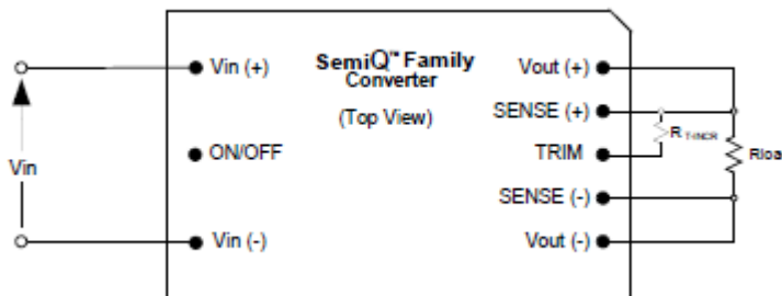
Figure 3. Configuration for increasing output voltage
