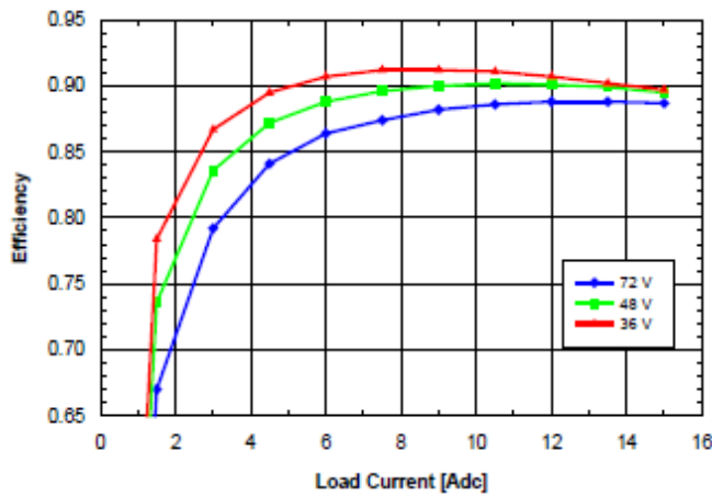
Fig. 2.5V.5: Efficiency vs. load current and input voltage for SQ48T/S15025 converter mounted vertically with air flowing from pin 3 to pin 1 at a rate of 300LFM (1.5 m/s) and T_a = 25^\circ\text{C} .
