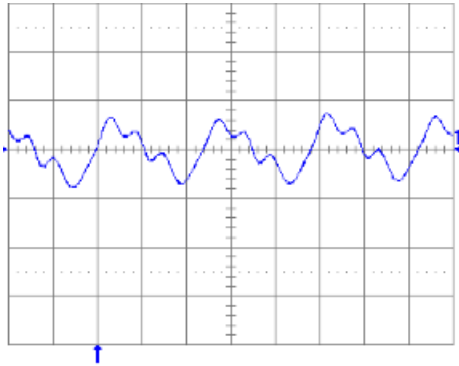
Fig.3.3V.13: Output voltage ripple (20 mV/div.) at full rated load current into a resistive load with C_o = 10\mu\text{F} tantalum + 1\mu\text{F} ceramic and V_{in} = 48\text{V} . Time scale: 1\mu\text{s}/\text{div} .
