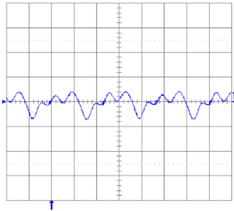
Fig. 2.0V.13: Output voltage ripple (20 mV/div.) at full rated load current into a resistive load with C_o = 10\mu\text{F} tantalum + 1\mu\text{F} ceramic and V_{in} = 48\text{V} . Time scale: 1\mu\text{s}/\text{div} .
