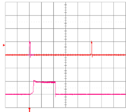
Fig. 3.3V.18: Load current (top trace, 10\text{A}/\text{div.} , 20\text{ ms}/\text{div.} ) into a 10\text{ m}\Omega short circuit during restart, at V_{in} = 48\text{V} . Bottom trace ( 20\text{A}/\text{div.} , 1\text{ ms}/\text{div.} ) is an expansion of the on-time portion of the top trace.
