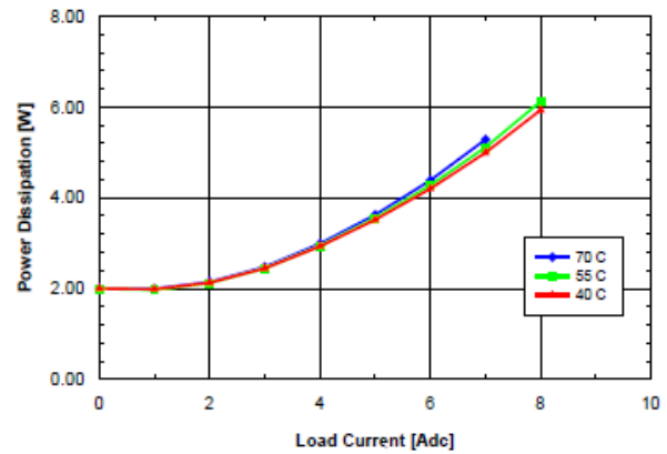
Fig. 6.0V.6: Power dissipation vs. load current and ambient temperature for SQ48T/S08060 converter mounted vertically with V_{in} = 48\text{V} and air flowing from pin 3 to pin 1 at a rate of 200LFM (1.0m/s).
