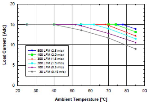
Figure 3.3V.1 Available load current vs. ambient air temperature and airflow rates for SQ48T15033 converter with D height pins mounted vertically with V_{in} = 48V , air flowing from pin 3 to pin 1, and maximum FET temperature \leq 120^{\circ}C .
