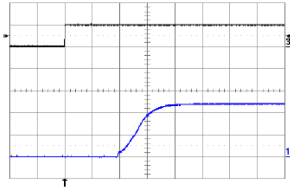
Fig. 12V.7: Turn-on transient at full rated load current (resistive) with no output capacitor at V_{in} = 48\text{V} , triggered via ON/OFF pin. Top trace: ON/OFF signal 5V/div.). Bottom trace: output voltage (5V/div.). Time scale: 1ms/div.
