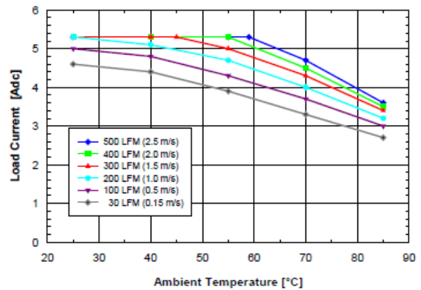
Figure 8.0V.2 Available load current vs. ambient air temperature and airflow rates for SQ48T05080 converter with D height pins mounted horizontally with V_{in} = 48V , air flowing from pin 3 to pin 1, and maximum FET temperature \leq 120^{\circ}C .
