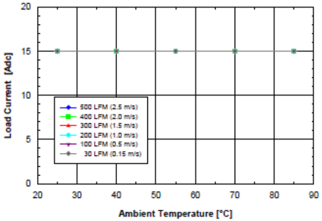
Figure 1.0V.4 Available load current vs. ambient air temperature and airflow rates for SQ48S15010 converter with D height pins mounted horizontally with V_{in} = 48V , air flowing from pin 3 to pin 1, and maximum FET temperature \leq 120^{\circ}C .
