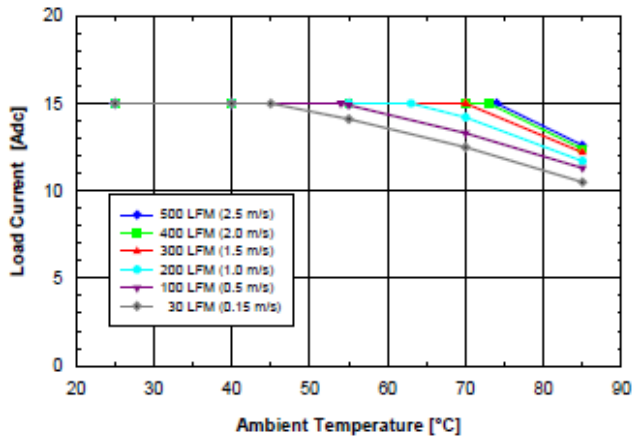
Figure 2.5V.4 Available load current vs. ambient air temperature and airflow rates for SQ48S15025 converter with D height pins mounted horizontally with V_{in} = 48V , air flowing from pin 3 to pin 1, and maximum FET temperature \leq 120^{\circ}C .
