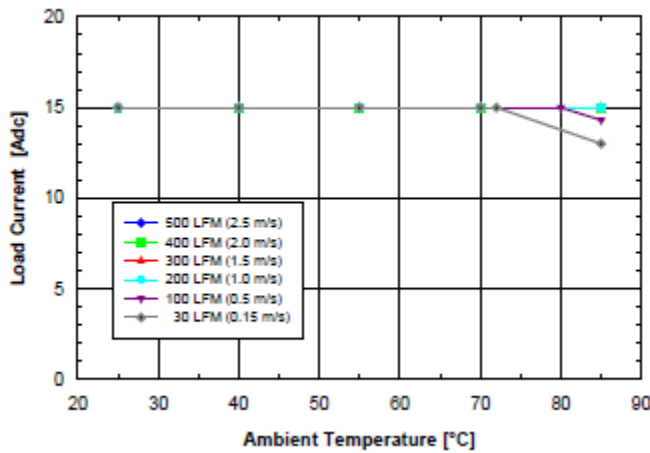
Figure 1.2V.1 Available load current vs. ambient air temperature and airflow rates for SQ48T15012 converter with D height pins mounted vertically with V_{in} = 48V , air flowing from pin 3 to pin 1, and maximum FET temperature \leq 120^{\circ}C .
