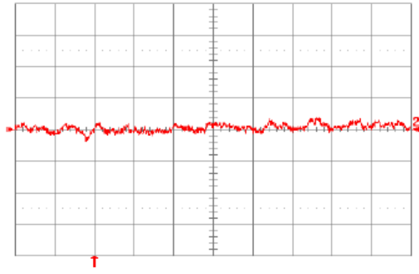
Fig. 12V.14: Input reflected ripple current, i_s (100 mA/div.), measured at input terminals at full rated full rated load current and V_{in} = 48V . Refer to Fig. 12V.14 for test setup. Time scale: 1 \mu s/div.
