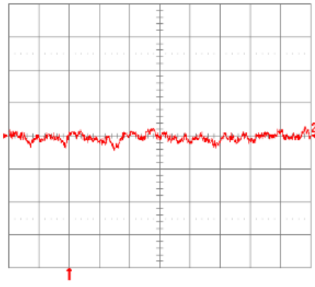
Fig. 1.8V.16: Input reflected ripple current, i_s (10 mA/div.), measured through 10\mu\text{H} at the source at full rated full rated load current and V_{in} = 48\text{V} . Refer to Fig. 1.8V.14 for test setup. Time scale: 1\mu\text{s}/\text{div} .
