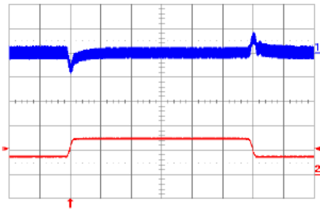
Fig. 1.0V.11: Output voltage response to load current step-change (3.75 A – 7.5 A – 3.75 A) at V_{in} = 48V . Top trace: output voltage (100mV/div.). Bottom trace: load current (5A/div.). Current slew rate: 0.1A/ \mu s . C_o = 1\mu F ceramic. Time scale: 0.2 ms/div.
