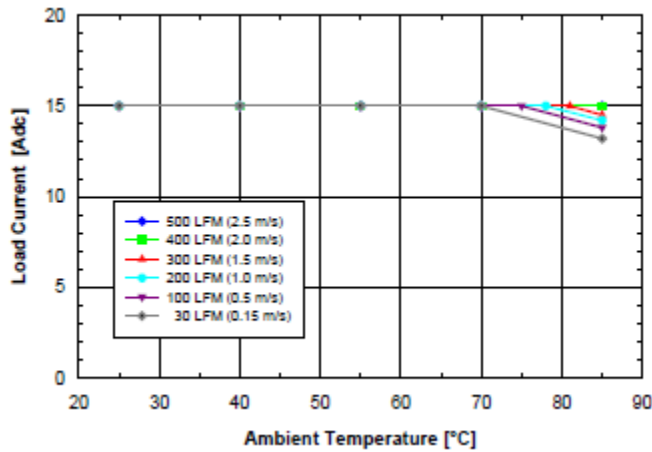
Figure 1.8V.3 Available load current vs. ambient air temperature and airflow rates for SQ48S15018 converter with D height pins mounted vertically with V_{in} = 48V , air flowing from pin 3 to pin 1, and maximum FET temperature \leq 120^{\circ}C .
