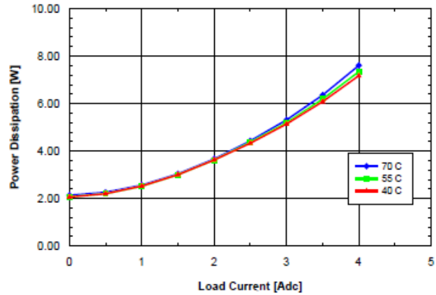
Fig. 12V.6: Power dissipation vs. load current and ambient temperature for SQ48T/S04120 converter mounted vertically with V_{in} = 48\text{V} and air flowing from pin 3 to pin 1 at a rate of 200LFM (1.0m/s).
