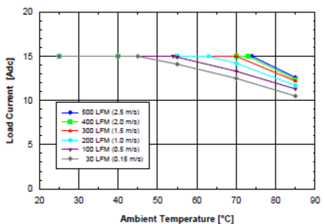
Figure 3.3V.4 Available load current vs. ambient air temperature and airflow rates for SQ48S15033 converter with D height pins mounted horizontally with V_{in} = 48V , air flowing from pin 3 to pin 1, and maximum FET temperature \leq 120^{\circ}C .
