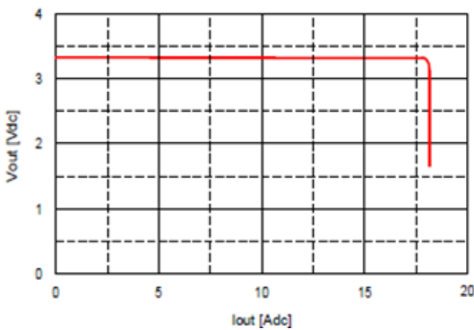
Fig. 3.3V.17: Output voltage vs. load current showing current limit point and converter shutdown point. Input voltage has almost no effect on current limit characteristic.
