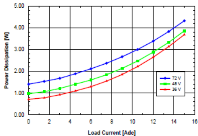
Fig. 1.2V.7: Power dissipation vs. load current and input voltage for SQ48T/S15012 converter mounted vertically with air flowing from pin 3 to pin 1 at a rate of 300 LFM (1.5 m/s) and T_a = 25^\circ\text{C} .
