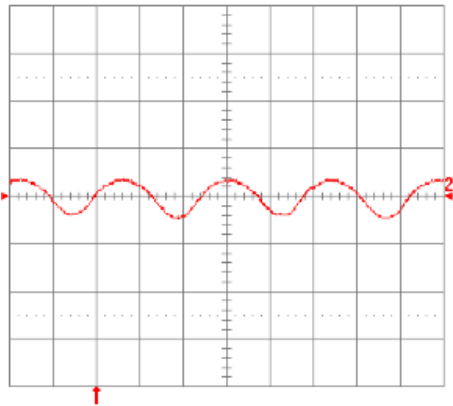
Fig. 1.8V.15: Input reflected ripple current, i_c (100 mA/div.), measured at input terminals at full rated load current and V_{in} = 48\text{V} . Refer to Fig. 1.8V.14 for test setup. Time scale: 1\mu\text{s}/\text{div} .
