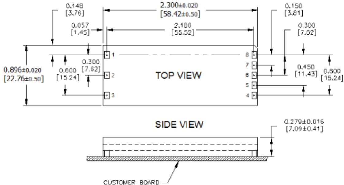
SQ48T Pinout (Through-hole)
