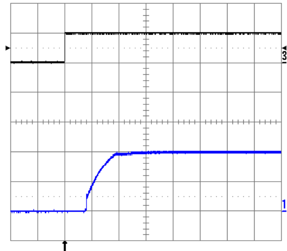
Fig. 2.0V.10: Turn-on transient at full rated load current (resistive) plus 10,000 \mu F at V_{in} = 48V , triggered via ON/OFF pin. Top trace: ON/OFF signal (5V/div.). Bottom trace: output voltage (1V/div.). Time scale: 2ms/div.
