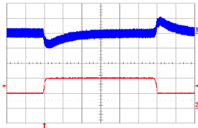
Fig. 6.0V.9: Output voltage response to load current step-change (2 A – 4 A – 2 A) at V_{in} = 48V . Top trace: output voltage (100mV/div.). Bottom trace: load current (2A/div.). Current slew rate: 0.1A/\mu s . C_o = 1\mu F ceramic. Time scale: 0.2 ms/div.
