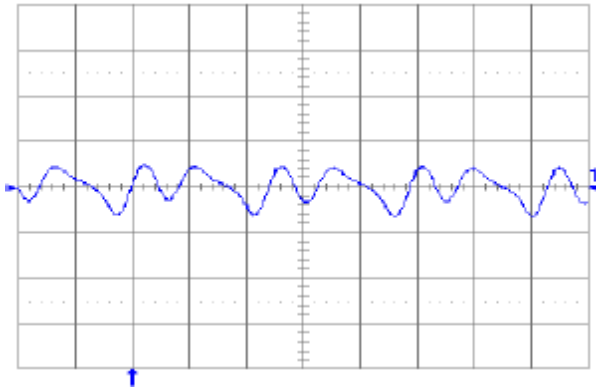
Fig. 1.0V.13: Output voltage ripple (20 mV/div.) at full rated load current into a resistive load with C_o = 10\mu\text{F} tantalum + 1\mu\text{F} ceramic and V_{in} = 48\text{V} . Time scale: 1\mu\text{s}/\text{div} .
