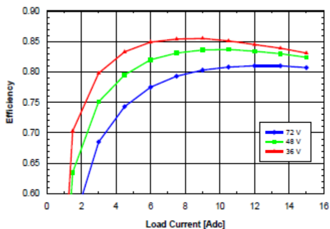
Fig. 1.2V.5: Efficiency vs. load current and input voltage for SQ48T/S15012 converter mounted vertically with air flowing from pin 3 to pin 1 at a rate of 300LFM (1.5 m/s) and T_a = 25^\circ\text{C} .
