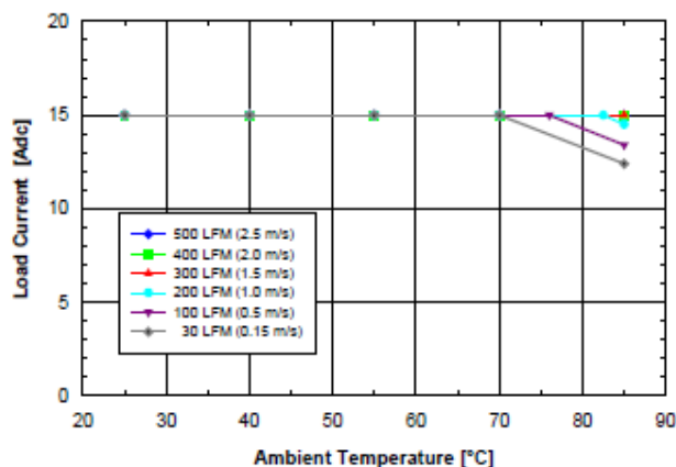
Figure 1.5V.1 Available load current vs. ambient air temperature and airflow rates for SQ48T15015 converter with D height pins mounted vertically with V_{in} = 48V , air flowing from pin 3 to pin 1, and maximum FET temperature \leq 120^{\circ}C .
