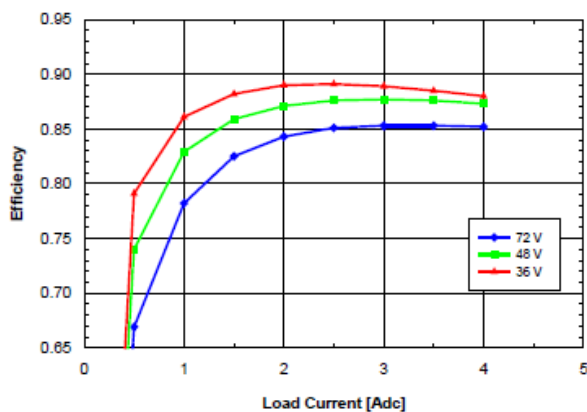
Fig. 12V.3: Efficiency vs. load current and input voltage for SQ48T/S04120 converter mounted vertically with air flowing from pin 3 to pin 1 at a rate of 300LFM (1.5 m/s) and T_a = 25^{\circ}C .
