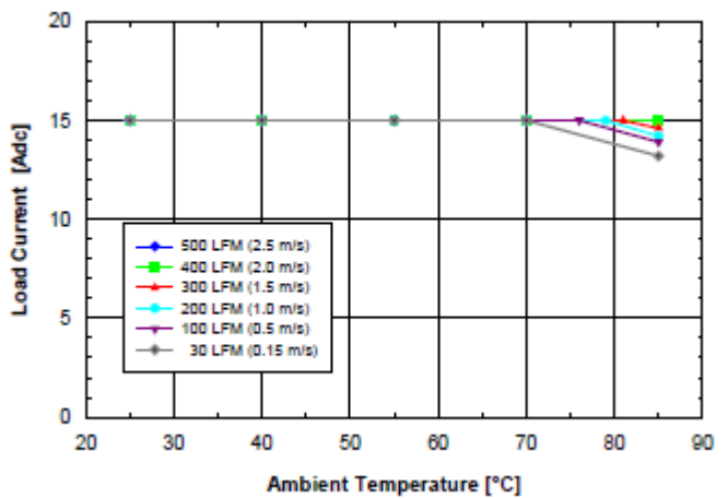
Figure 1.8V.4 Available load current vs. ambient air temperature and airflow rates for SQ48S15018 converter with D height pins mounted horizontally with V_{in} = 48V , air flowing from pin 3 to pin 1, and maximum FET temperature \leq 120^{\circ}C .
