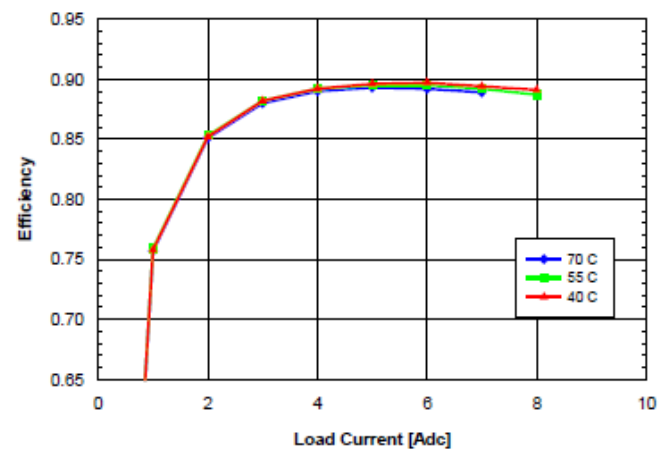
Fig. 6.0V.4: Efficiency vs. load current and ambient temperature for SQ48T/S08060 converter mounted vertically with V_{in} = 48V and air flowing from pin 3 to pin 1 at a rate of 200LFM (1.0 m/s).
