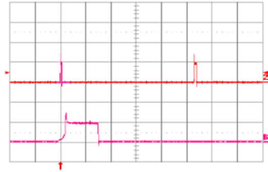
Fig. 1.8V.18: Load current (top trace, 20A/div., 20 ms/div.) into a 10\text{m}\Omega short circuit during restart, at V_{in} = 48\text{V} . Bottom trace (20A/div., 1ms/div.) is an expansion of the on-time portion of the top trace.
