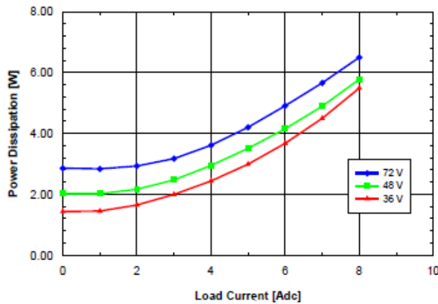
Fig. 6.0V.5: Power dissipation vs. load current and input voltage for SQ48T/S08060 converter mounted vertically with air flowing from pin 3 to pin 1 at a rate of 300 LFM (1.5 m/s) and T_a = 25^\circ\text{C} .
