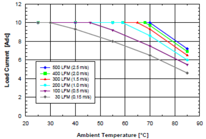
Figure 5.0V.2 Available load current vs. ambient air temperature and airflow rates for SQ48T10050 converter with D height pins mounted horizontally with V_{in} = 48V , air flowing from pin 3 to pin 1, and maximum FET temperature \leq 120^{\circ}C .
