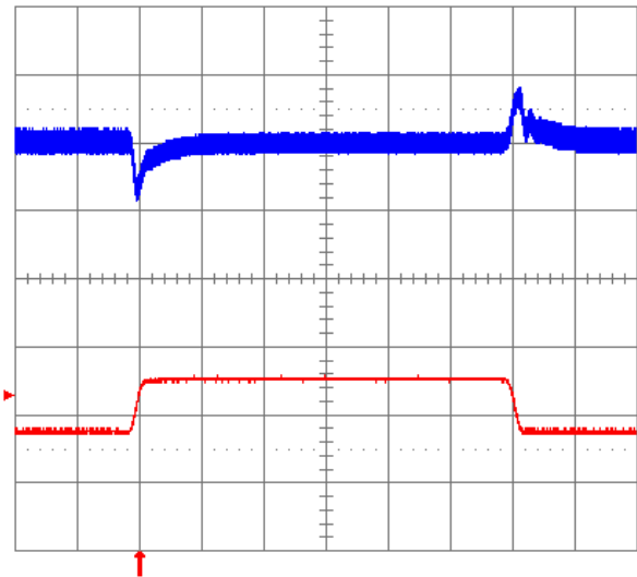
Fig. 1.5V.11: Output voltage response to load current step-change (3.75 A – 7.5 A – 3.75 A) at V_{in} = 48V . Top trace: output voltage (100mV/div.). Bottom trace: load current (5A/div.). Current slew rate: 0.1A/ \mu s . C_o = 1\mu F ceramic. Time scale: 0.2 ms/div.
