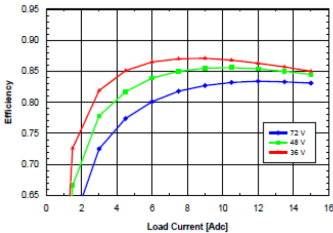
Fig. 1.5V.5: Efficiency vs. load current and input voltage for SQ48T/S15015 converter mounted vertically with air flowing from pin 3 to pin 1 at a rate of 300LFM (1.5 m/s) and T_a = 25^\circ\text{C} .
