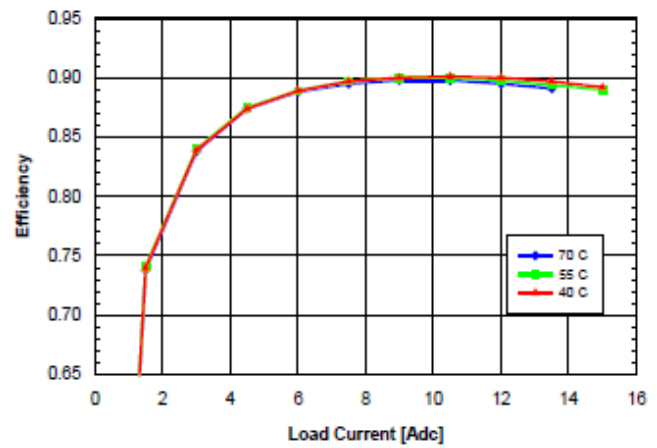
Fig. 2.5V.6: Efficiency vs. load current and ambient temperature for SQ48T/S15025 converter mounted vertically with V_{in} = 48\text{V} and air flowing from pin 3 to pin 1 at a rate of 200LFM (1.0 m/s).
