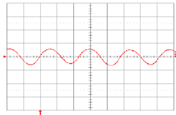
Fig. 5.0V.15: Input reflected ripple current, i_c (100 mA/div.), measured at input terminals at full rated load current and V_{in} = 48\text{V} . Refer to Fig. 5.0V.14 for test setup. Time scale: 1\mu\text{s}/\text{div} .
