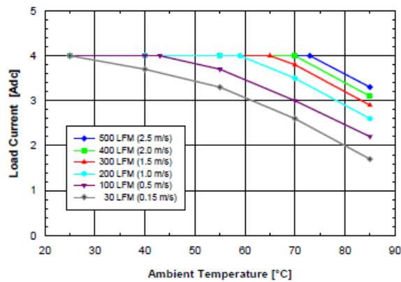
Figure 12V.1 Available load current vs. ambient air temperature and airflow rates for SQ48T04120 converter with D height pins mounted vertically with V_{in} = 48V , air flowing from pin 3 to pin 1, and maximum FET temperature \leq 120^{\circ}C .
