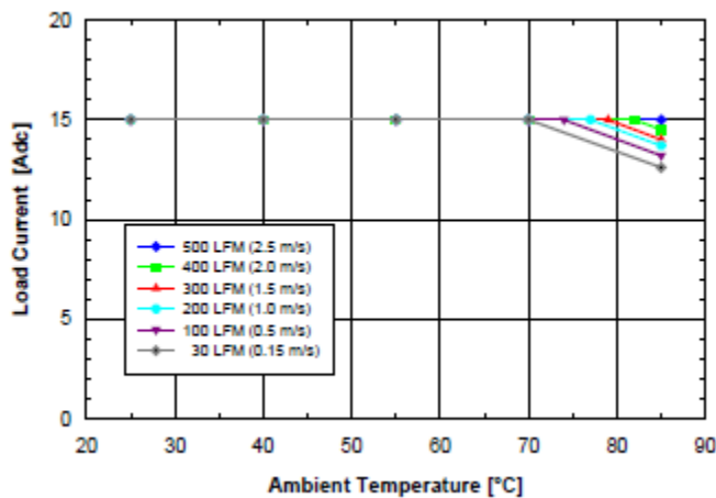
Figure 2.0V.3 Available load current vs. ambient air temperature and airflow rates for SQ48S15020 converter with D height pins mounted vertically with V_{in} = 48V , air flowing from pin 3 to pin 1, and maximum FET temperature \leq 120^{\circ}C .
