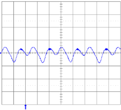
Fig. 1.5V.13: Output voltage ripple (20 mV/div.) at full rated load current into a resistive load with C_o = 10\mu\text{F} tantalum + 1\mu\text{F} ceramic and V_{in} = 48\text{V} . Time scale: 1\mu\text{s}/\text{div} .
