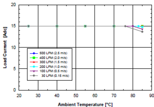
Figure 1.5V.3 Available load current vs. ambient air temperature and airflow rates for SQ48S15015 converter with D height pins mounted vertically with V_{in} = 48V , air flowing from pin 3 to pin 1, and maximum FET temperature \leq 120^{\circ}C .
