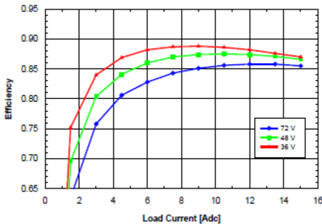
Fig. 2.0V.5: Efficiency vs. load current and input voltage for SQ48T/S15020 converter mounted vertically with air flowing from pin 3 to pin 1 at a rate of 300LFM (1.5 m/s) and T_a = 25^\circ\text{C} .
