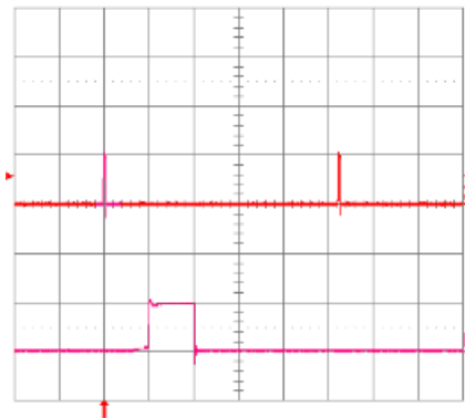
Fig. 1.5V.18: Load current (top trace, 20A/div., 20 ms/div.) into a 10\text{ m}\Omega short circuit during restart, at V_{in} = 48\text{V} . Bottom trace (20A/div., 1ms/div.) is an expansion of the on-time portion of the top trace.
