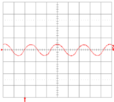
Fig. 2.5V.15: Input reflected ripple current, i_c (100 mA/div.), measured at input terminals at full rated load current and V_{in} = 48\text{V} . Refer to Fig. 2.5V.14 for test setup. Time scale: 1\mu\text{s}/\text{div} .
