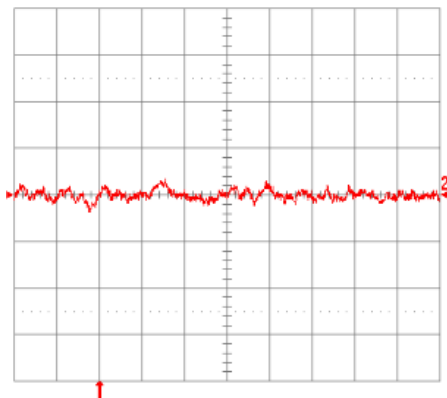
Fig. 2.5V.16: Input reflected ripple current, i_s (10 mA/div.), measured through 10\mu\text{H} at the source at full rated full rated load current and V_{in} = 48\text{V} . Refer to Fig. 2.5V.14 for test setup. Time scale: 1\mu\text{s}/\text{div} .
