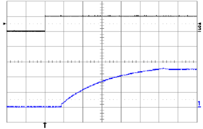
Fig. 5.0V.10: Turn-on transient at full rated load current (resistive) plus 10,000 \mu F at V_{in} = 48V , triggered via ON/OFF pin. Top trace: ON/OFF signal (5V/div.). Bottom trace: output voltage (2V/div.). Time scale: 5ms/div.
