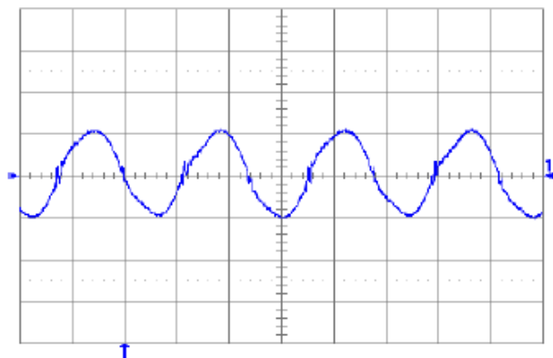
Fig. 5.0V.13: Output voltage ripple (20 mV/div.) at full rated load current into a resistive load with C_o = 10\mu\text{F} tantalum + 1\mu\text{F} ceramic and V_{in} = 48\text{V} . Time scale: 1\mu\text{s}/\text{div} .
