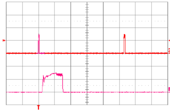
Fig. 6.0V.16: Load current (top trace, 10A/div., 20 ms/div.) into a 10 m \Omega short circuit during restart, at V_{in} = 48V . Bottom trace (10A/div., 1ms/div.) is an expansion of the on-time portion of the top trace.
