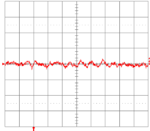
Fig. 3.3V.16: Input reflected ripple current, i_s (10 mA/div.), measured through 10\mu\text{H} at the source at full rated full rated load current and V_{in} = 48\text{V} . Refer to Fig. 3.3V.14 for test setup. Time scale: 1\mu\text{s}/\text{div} .
