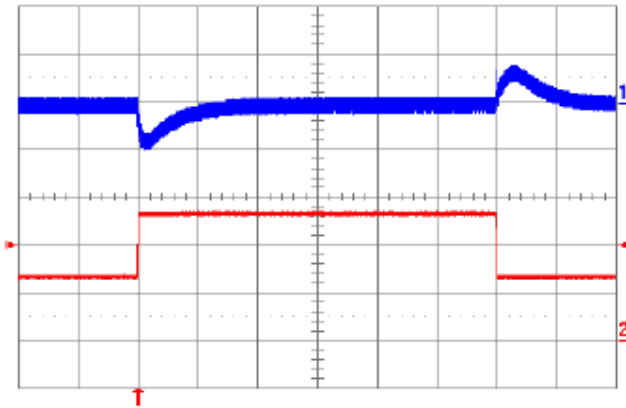
Fig. 8.0V.9: Output voltage response to load current step-change (1.325A – 2.65A – 1.325A) at V_{in} = 48V . Top trace: output voltage (200mV/div.). Bottom trace: load current (1A/div.). Current slew rate: 0.1A/ \mu s. C_o = 1\mu F ceramic. Time scale: 0.5 ms/div.
