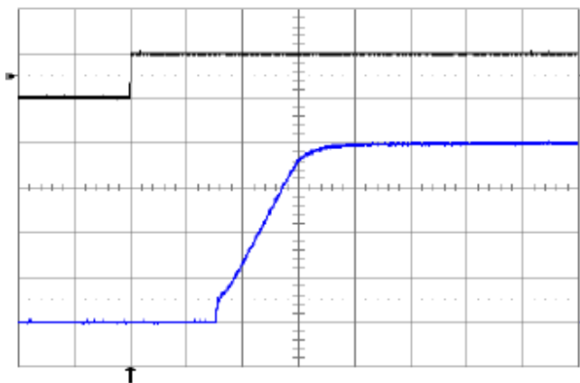
Fig. 8.0V.7: Turn-on transient at full rated load current (resistive) with no output capacitor at V_{in} = 48\text{V} , triggered via ON/OFF pin. Top trace: ON/OFF signal (5V/div.). Bottom trace: output voltage (2V/div.). Time scale: 1ms/div.
