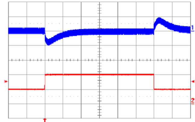
Fig. 12V.10: Output voltage response to load current step-change (1A – 2A – 1A) at V_{in} = 48V . Top trace: output voltage (200 mV/div.). Bottom trace: load current (1A/div.). Current slew rate: 5 A/ \mu s. C_o = 47\mu F tantalum + 1 \mu F ceramic. Time scale: 0.5 ms/div.
