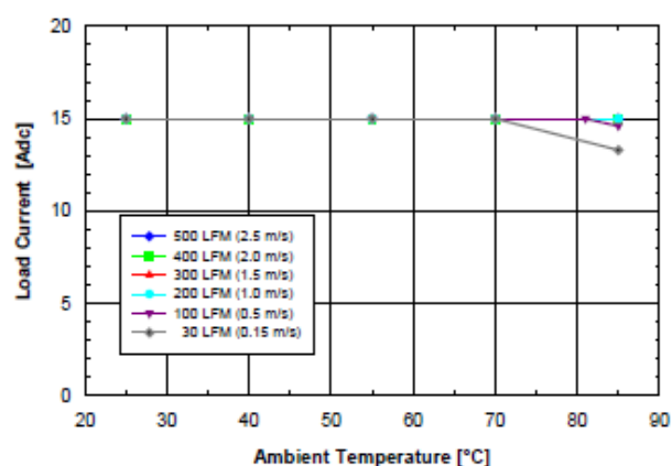
Figure 1.5V.2 Available load current vs. ambient air temperature and airflow rates for SQ48T15015 converter with D height pins mounted horizontally with V_{in} = 48V , air flowing from pin 3 to pin 1, and maximum FET temperature \leq 120^{\circ}C .
