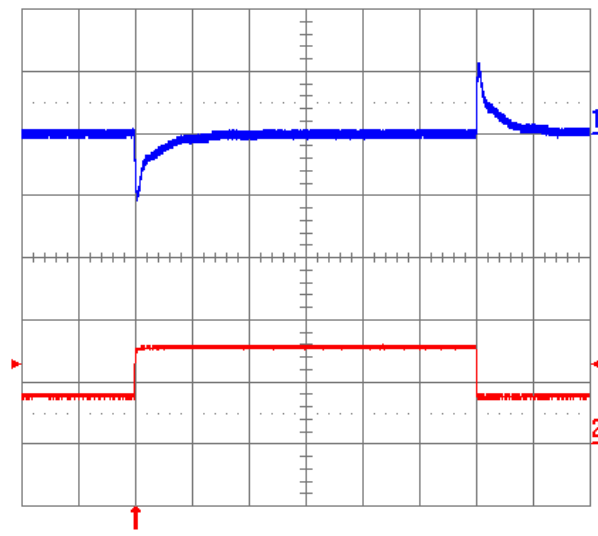
Fig. 2.5V.12: Output voltage response to load current step-change (3.75 A – 7.5 A – 3.75 A) at V_{in} = 48V . Top trace: output voltage (100 mV/div.). Bottom trace: load current (5A/div.). Current slew rate: 5 A/ \mu s . C_o = 450\mu F tantalum + 1 \mu F ceramic. Time scale: 0.2 ms/div.
