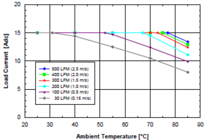
Figure 3.3V.2 Available load current vs. ambient air temperature and airflow rates for SQ48T15033 converter with D height pins mounted horizontally with V_{in} = 48V , air flowing from pin 3 to pin 1, and maximum FET temperature \leq 120^{\circ}C .
