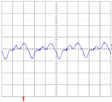
Fig. 1.8V.13: Output voltage ripple (20 mV/div.) at full rated load current into a resistive load with C_o = 10\mu\text{F} tantalum + 1\mu\text{F} ceramic and V_{in} = 48\text{V} . Time scale: 1\mu\text{s}/\text{div} .
