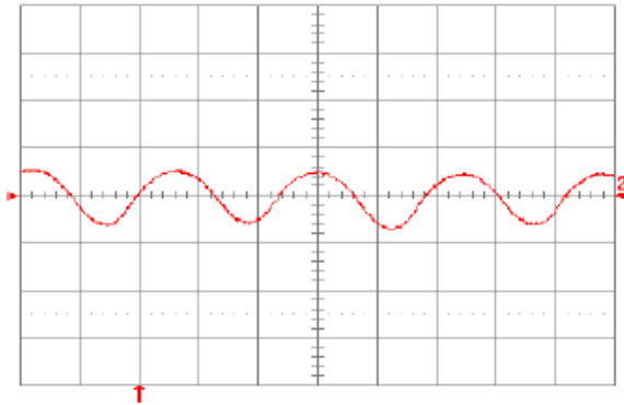
Fig. 6.0V.13: Input reflected ripple current, i_c (100 mA/div.), measured at input terminals at full rated load current and V_{in} = 48V . Refer to Fig. 6.0V.14 for test setup. Time scale: 1 \mu s/div.
