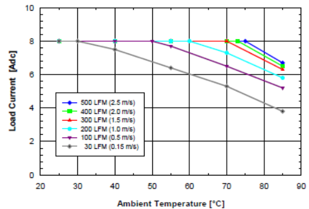
Figure 6.0V.2 Available load current vs. ambient air temperature and airflow rates for SQ48T08060 converter with D height pins mounted horizontally with V_{in} = 48V , air flowing from pin 3 to pin 1, and maximum FET temperature \leq 120^{\circ}C .
