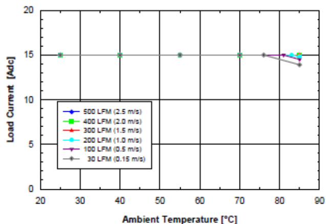
Figure 1.5V.4 Available load current vs. ambient air temperature and airflow rates for SQ48S15015 converter with D height pins mounted horizontally with V_{in} = 48V , air flowing from pin 3 to pin 1, and maximum FET temperature \leq 120^{\circ}C .
