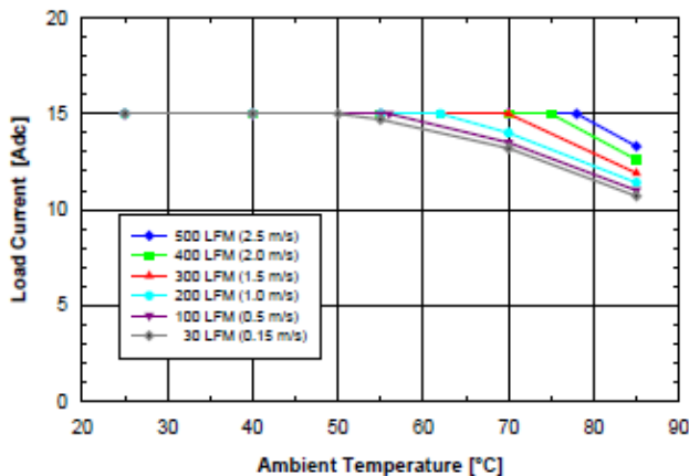
Figure 3.3V.3 Available load current vs. ambient air temperature and airflow rates for SQ48S15033 converter with D height pins mounted vertically with V_{in} = 48V , air flowing from pin 3 to pin 1, and maximum FET temperature \leq 120^{\circ}C .
