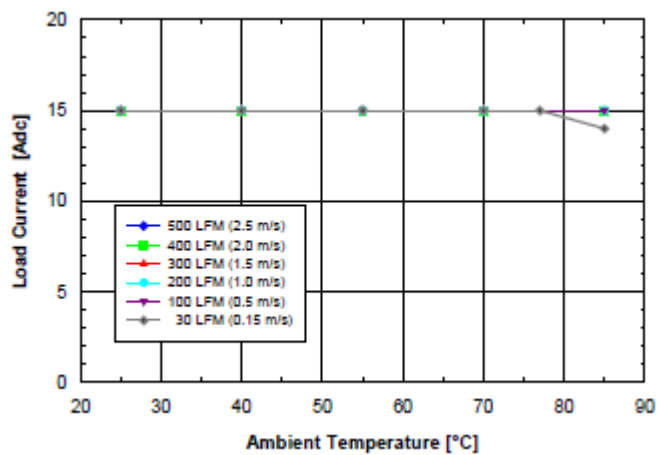
Figure 1.2V.2 Available load current vs. ambient air temperature and airflow rates for SQ48T15012 converter with D height pins mounted horizontally with V_{in} = 48V , air flowing from pin 3 to pin 1, and maximum FET temperature \leq 120^{\circ}C .
