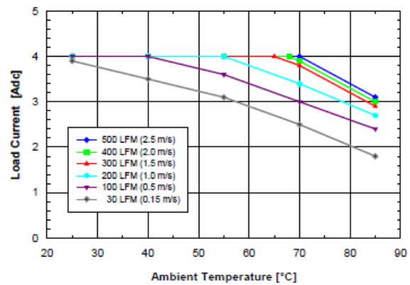
Figure 12V.2 Available load current vs. ambient air temperature and airflow rates for SQ48T04120 converter with D height pins mounted horizontally with V_{in} = 48V , air flowing from pin 3 to pin 1, and maximum FET temperature \leq 120^{\circ}C .
