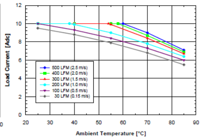
Figure 5.0V.4 Available load current vs. ambient air temperature and airflow rates for SQ48S10050 converter with D height pins mounted horizontally with V_{in} = 48V , air flowing from pin 3 to pin 1, and maximum FET temperature \leq 120^{\circ}C .
