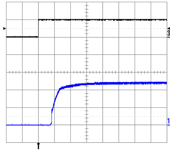
Fig. 1.2V.10: Turn-on transient at full rated load current (resistive) plus 10,000 \mu F at V_{in} = 48V , triggered via ON/OFF pin. Top trace: ON/OFF signal (5V/div.). Bottom trace: output voltage (0.5V/div.). Time scale: 2ms/div.
