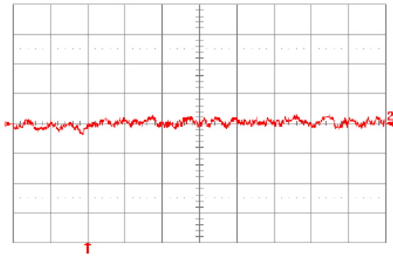
Fig. 8.0V.14: Input reflected ripple current, i_c (10 mA/div.), measured through 10 \mu H at the source at full rated full rated load current and V_{in} = 48V . Refer to Fig. 8.0V.14 for test setup. Time scale: 1 \mu s/div.
