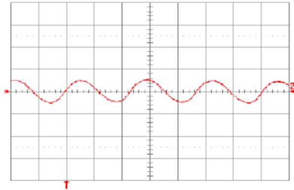
Fig. 12V.13: Input reflected ripple current, i_c (100 mA/div.), measured at input terminals at full rated load current and V_{in} = 48V . Refer to Fig. 12V.14 for test setup. Time scale: 1 \mu s/div.
