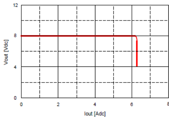
Fig. 8.0V.15: Output voltage vs. load current showing current limit point and converter shutdown point. Input voltage has almost no effect on current limit characteristic.
