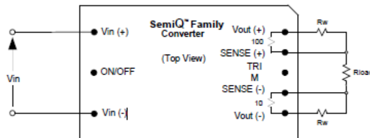
Figure 2. Remote sense circuit configuration
