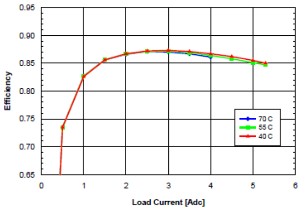
Fig. 8.0V.4: Efficiency vs. load current and ambient temperature for SQ48T/S05080 converter mounted vertically with V_{in} = 48V and air flowing from pin 3 to pin 1 at a rate of 200LFM (1.0 m/s).
