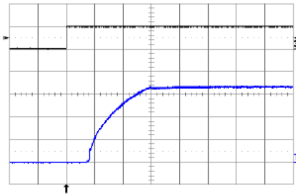
Fig. 3.3V.10: Turn-on transient at full rated load current (resistive) plus 10,000 \mu F at V_{in} = 48V , triggered via ON/OFF pin. Top trace: ON/OFF signal (5V/div.). Bottom trace: output voltage (1V/div.). Time scale: 2ms/div.
