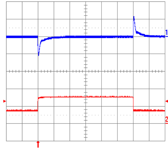
Fig. 1.2V.12: Output voltage response to load current step-change (3.75 A – 7.5 A – 3.75 A) at V_{in} = 48V . Top trace: output voltage (100 mV/div.). Bottom trace: load current (5A/div.). Current slew rate: 5 A/ \mu s . C_o = 450\mu F tantalum + 1\mu F ceramic. Time scale: 0.2 ms/div.
