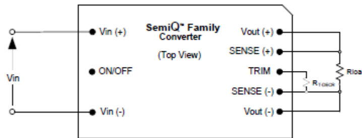
Figure 4. Configuration for decreasing output voltage
