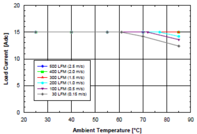
Figure 1.8V.2 Available load current vs. ambient air temperature and airflow rates for SQ48T15018 converter with D height pins mounted horizontally with V_{in} = 48V , air flowing from pin 3 to pin 1, and maximum FET temperature \leq 120^{\circ}C .
