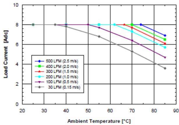
Figure 6.0V.1 Available load current vs. ambient air temperature and airflow rates for SQ48T08060 converter with D height pins mounted vertically with V_{in} = 48V , air flowing from pin 3 to pin 1, and maximum FET temperature \leq 120^{\circ}C .
