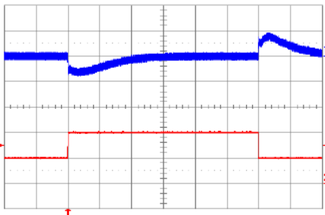
Fig. 6.0V.10: Output voltage response to load current step-change (2 A – 4 A – 2 A) at V_{in} = 48V . Top trace: output voltage (100 mV/div.). Bottom trace: load current (2A/div.). Current slew rate: 5 A/\mu s . C_o = 450\mu F tantalum + 1\mu F ceramic. Time scale: 0.2 ms/div.
