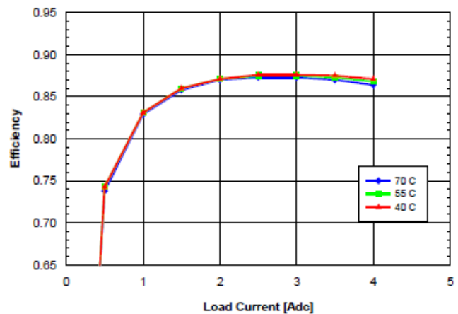
Fig. 12V.4: Efficiency vs. load current and ambient temperature for SQ48T/S04120 converter mounted vertically with V_{in} = 48V and air flowing from pin 3 to pin 1 at a rate of 200LFM (1.0 m/s).
