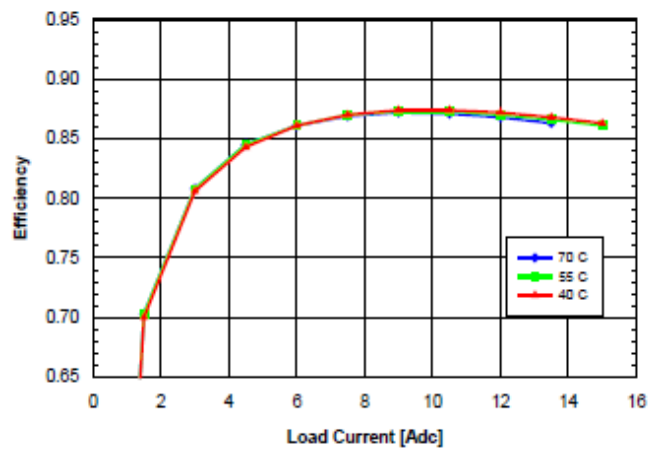
Fig. 2.0V.6: Efficiency vs. load current and ambient temperature for SQ48T/S15020 converter mounted vertically with V_{in} = 48\text{V} and air flowing from pin 3 to pin 1 at a rate of 200LFM (1.0 m/s).
