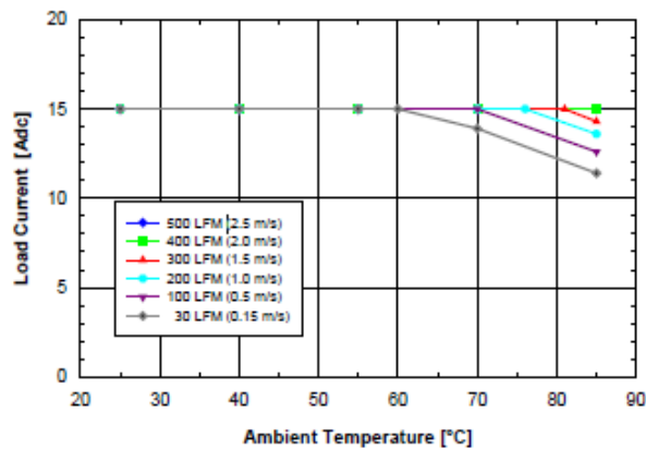
Figure 2.0V.1 Available load current vs. ambient air temperature and airflow rates for SQ48T15020 converter with D height pins mounted vertically with V_{in} = 48V , air flowing from pin 3 to pin 1, and maximum FET temperature \leq 120^{\circ}C .
