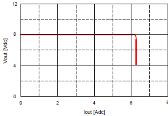
Fig. 6.0V.15: Output voltage vs. load current showing current limit point and converter shutdown point. Input voltage has almost no effect on current limit characteristic.
