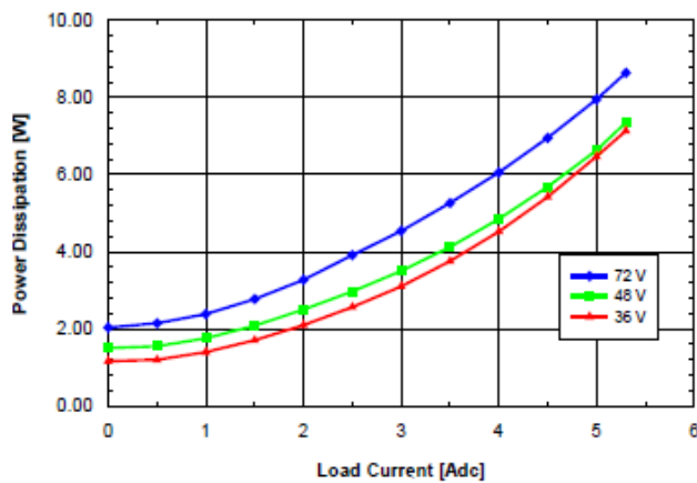
Fig. 8.0V.5: Power dissipation vs. load current and input voltage for SQ48T/S05080 converter mounted vertically with air flowing from pin 3 to pin 1 at a rate of 300 LFM (1.5 m/s) and T_a = 25^\circ\text{C} .
