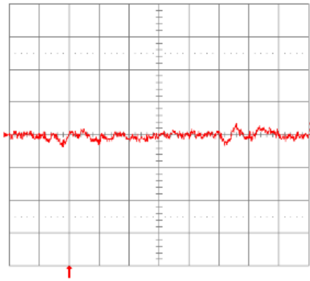
Fig. 1.2V.16: Input reflected ripple current, i_s (10 mA/div.), measured through 10\mu\text{H} at the source at full rated full rated load current and V_{in} = 48\text{V} . Refer to Fig. 1.2V.14 for test setup. Time scale: 1\mu\text{s}/\text{div} .
