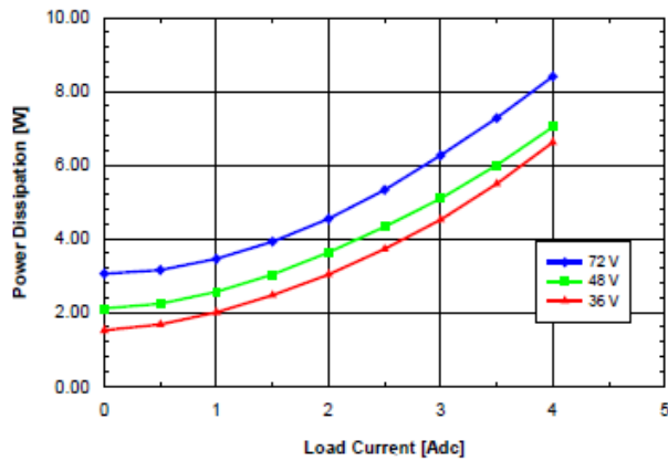
Fig. 12V.5: Power dissipation vs. load current and input voltage for SQ48T/S04120 converter mounted vertically with air flowing from pin 3 to pin 1 at a rate of 300 LFM (1.5 m/s) and T_a = 25^\circ\text{C} .
