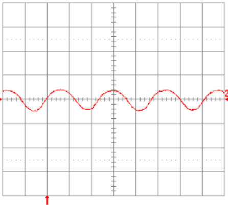
Fig. 2.0V.15: Input reflected ripple current, i_c (100 mA/div.), measured at input terminals at full rated load current and V_{in} = 48\text{V} . Refer to Fig. 2.0V.14 for test setup. Time scale: 1\mu\text{s}/\text{div} .
