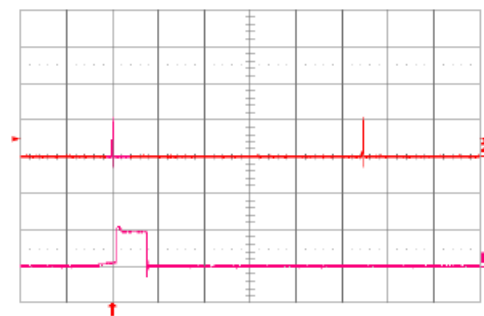
Fig. 2.0V.16: Input reflected ripple current, i_s (10 mA/div.), measured through 10\mu\text{H} at the source at full rated full rated load current and V_{in} = 48\text{V} . Refer to Fig. 2.0V.14 for test setup. Time scale: 1\mu\text{s}/\text{div} .
