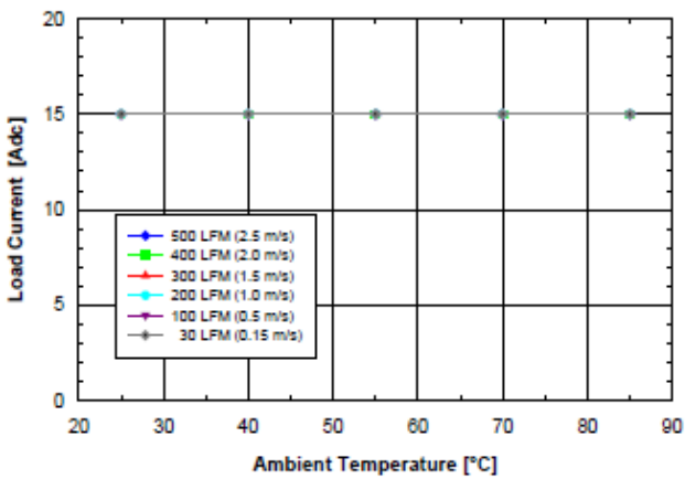
Figure 1.0V.3 Available load current vs. ambient air temperature and airflow rates for SQ48S15010 converter with D height pins mounted vertically with V_{in} = 48V , air flowing from pin 3 to pin 1, and maximum FET temperature \leq 120^{\circ}C .
