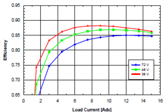
Fig. 1.8V.5: Efficiency vs. load current and input voltage for SQ48T/S15018 converter mounted vertically with air flowing from pin 3 to pin 1 at a rate of 300LFM (1.5 m/s) and T_a = 25^\circ\text{C} .
