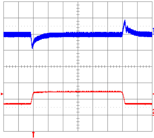
Fig. 1.8V.11: Output voltage response to load current step-change (3.75 A - 7.5 A - 3.75 A) at V_{in} = 48V . Top trace: output voltage (100mV/div.). Bottom trace: load current (5A/div.). Current slew rate: 0.1A/ \mu s . C_o = 1\mu F ceramic. Time scale: 0.2 ms/div.
