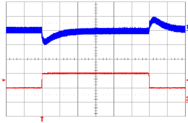
Fig. 12V.9: Output voltage response to load current step-change (1A – 2A – 1A) at V_{in} = 48V . Top trace: output voltage (200mV/div.). Bottom trace: load current (1A/div.). Current slew rate: 0.1A/ \mu s. C_o = 1\mu F ceramic. Time scale: 0.5 ms/div.
