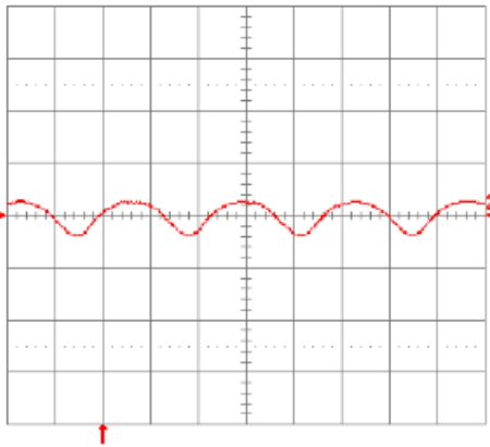
Fig. 1.2V.15: Input reflected ripple current, i_c (100 mA/div.), measured at input terminals at full rated load current and V_{in} = 48\text{V} . Refer to Fig. 1.2V.14 for test setup. Time scale: 1\mu\text{s}/\text{div} .
