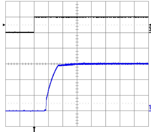
Fig. 1.5V.10: Turn-on transient at full rated load current (resistive) plus 10,000 \mu F at V_{in} = 48V , triggered via ON/OFF pin. Top trace: ON/OFF signal (5V/div.). Bottom trace: output voltage (0.5V/div.). Time scale: 2ms/div.
