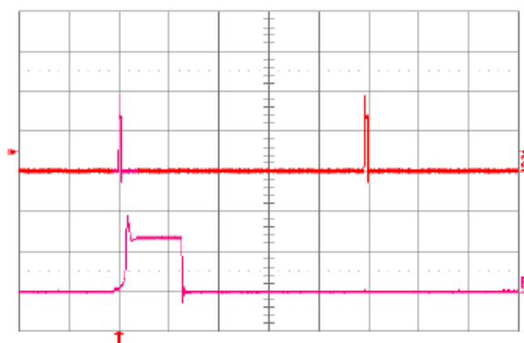
Fig. 5.0V.18: Load current (top trace, 10A/div., 20 ms/div.) into a 10\text{ m}\Omega short circuit during restart, at V_{in} = 48\text{V} . Bottom trace (10A/div., 1ms/div.) is an expansion of the on-time portion of the top trace.
