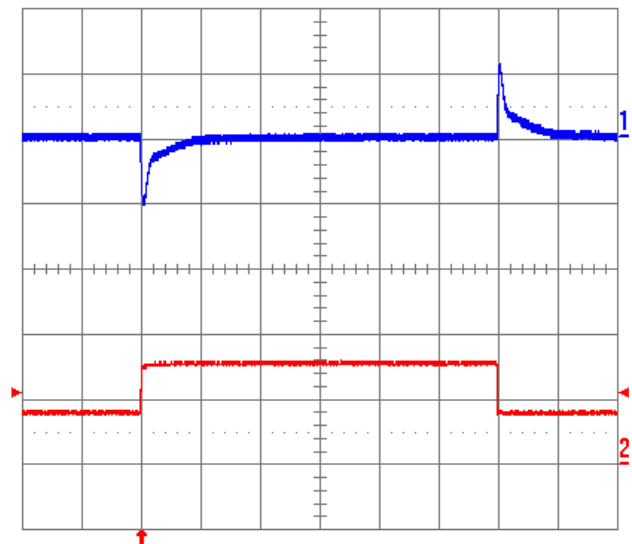
Fig. 2.0V.12: Output voltage response to load current step-change (3.75 A - 7.5 A - 3.75 A) at V_{in} = 48V . Top trace: output voltage (100 mV/div.). Bottom trace: load current (5A/div.). Current slew rate: 5 A/ \mu s . C_o = 450\mu F tantalum + 1 \mu F ceramic. Time scale: 0.2 ms/div.
