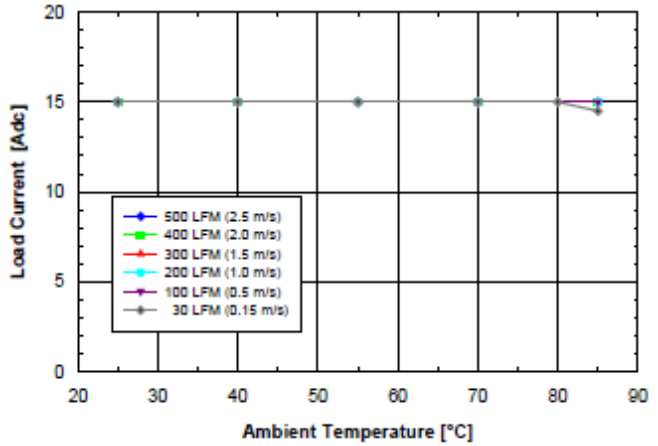
Figure 1.0V.2 Available load current vs. ambient air temperature and airflow rates for SQ48T15010 converter with D height pins mounted horizontally with V_{in} = 48V , air flowing from pin 3 to pin 1, and maximum FET temperature \leq 120^{\circ}C .
