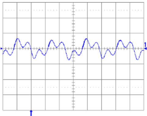
Fig. 2.5V.13: Output voltage ripple (20 mV/div.) at full rated load current into a resistive load with C_o = 10\mu\text{F} tantalum + 1\mu\text{F} ceramic and V_{in} = 48\text{V} . Time scale: 1\mu\text{s}/\text{div} .
