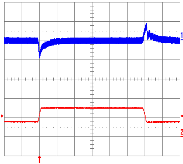
Fig. 2.0V.11: Output voltage response to load current step-change (3.75 A - 7.5 A - 3.75 A) at V_{in} = 48V . Top trace: output voltage (100mV/div.). Bottom trace: load current (5A/div.). Current slew rate: 0.1 A/ \mu s . C_o = 1\mu F ceramic. Time scale: 0.2 ms/div.
