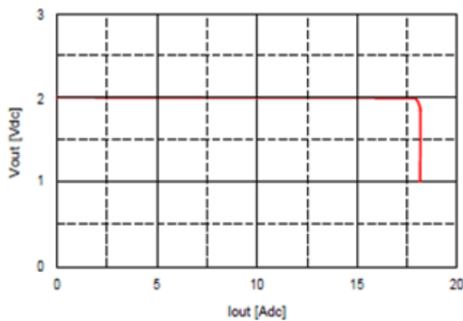
Fig. 2.0V.17: Output voltage vs. load current showing current limit point and converter shutdown point. Input voltage has almost no effect on current limit characteristic.
