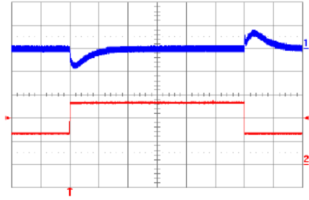
Fig. 8.0V.10: Output voltage response to load current step-change (1.325A – 2.65A – 1.325A) at V_{in} = 48V . Top trace: output voltage (200 mV/div.). Bottom trace: load current (1A/div.). Current slew rate: 5 A/ \mu s. C_o = 94\mu F tantalum + 1\mu F ceramic. Time scale: 0.5 ms/div.
