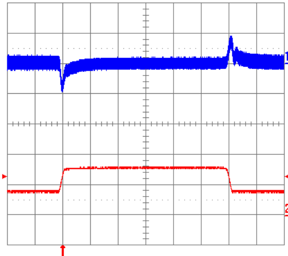
Fig. 1.2V.11: Output voltage response to load current step-change (3.75 A – 7.5 A – 3.75 A) at V_{in} = 48V . Top trace: output voltage (100mV/div.). Bottom trace: load current (5A/div.). Current slew rate: 0.1A/ \mu s . C_o = 1\mu F ceramic. Time scale: 0.2 ms/div.
