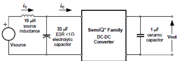
Fig. 6.0V.12: Test Setup for measuring input reflected ripple currents, i_c and i_s
