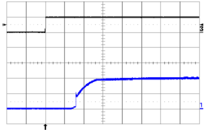
Fig. 1.0V.10: Turn-on transient at full rated load current (resistive) plus 10,000 \mu F at V_{in} = 48V , triggered via ON/OFF pin. Top trace: ON/OFF signal (5V/div.). Bottom trace: output voltage (0.5V/div.). Time scale: 2ms/div.
