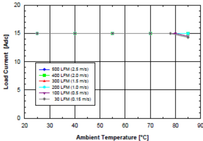
Figure 1.2V.3 Available load current vs. ambient air temperature and airflow rates for SQ48S15012 converter with D height pins mounted vertically with V_{in} = 48V , air flowing from pin 3 to pin 1, and maximum FET temperature \leq 120^{\circ}C .
