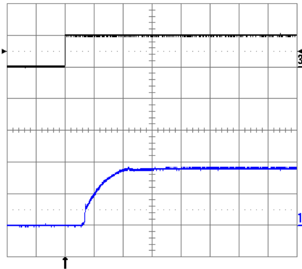
Fig. 1.8V.10: Turn-on transient at full rated load current (resistive) plus 10,000 \mu F at V_{in} = 48V , triggered via ON/OFF pin. Top trace: ON/OFF signal (5V/div.). Bottom trace: output voltage (1V/div.). Time scale: 2ms/div.
