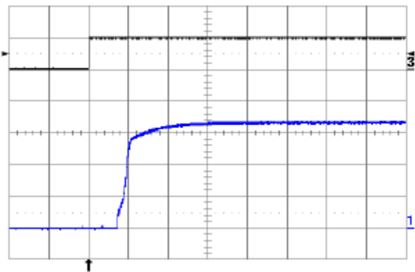
Fig. 3.3V.9: Turn-on transient at full rated load current (resistive) with no output capacitor at V_{in} = 48V , triggered via ON/OFF pin. Top trace: ON/OFF signal 5V/div.). Bottom trace: output voltage (2V/div.). Time scale: 2ms/div.
