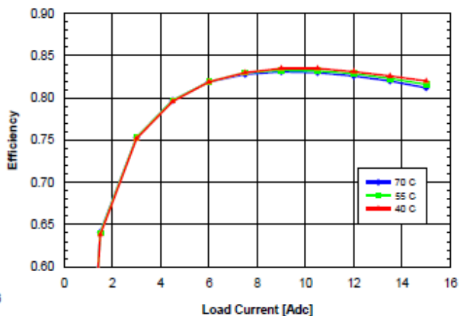
Fig. 1.2V.6: Efficiency vs. load current and ambient temperature for SQ48T/S15012 converter mounted vertically with V_{in} = 48\text{V} and air flowing from pin 3 to pin 1 at a rate of 200LFM (1.0 m/s).
