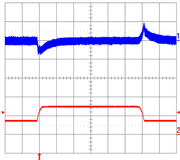
Fig. 3.3V.11: Output voltage response to load current step-change (3.75 A - 7.5 A - 3.75 A) at V_{in} = 48V . Top trace: output voltage (100mV/div.). Bottom trace: load current (5A/div.). Current slew rate: 0.1A/ \mu s . C_o = 1\mu F ceramic. Time scale: 0.2 ms/div.
