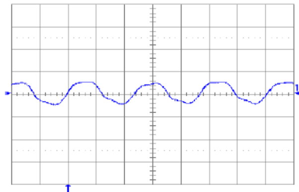
Fig.6.0V.11: Output voltage ripple (50 mV/div.) at full rated load current into a resistive load with C_o = 10\mu F tantalum + 1\mu F ceramic and V_{in} = 48V . Time scale: 1\mu s /div.
