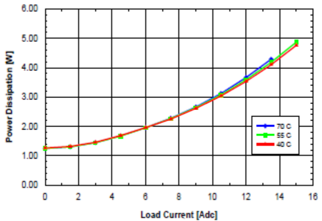
Fig. 2.0V.8: Power dissipation vs. load current and ambient temperature for SQ48T/S15020 converter mounted vertically with V_{in} = 48\text{V} and air flowing from pin 3 to pin 1 at a rate of 200LFM (1.0m/s).
