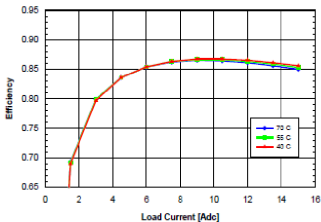
Fig. 1.8V.6: Efficiency vs. load current and ambient temperature for SQ48T/S15018 converter mounted vertically with V_{in} = 48\text{V} and air flowing from pin 3 to pin 1 at a rate of 200LFM (1.0 m/s).
