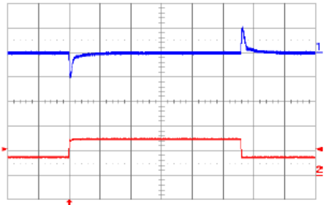
Fig. 1.0V.12: Output voltage response to load current step-change (3.75 A – 7.5 A – 3.75 A) at V_{in} = 48V . Top trace: output voltage (100 mV/div.). Bottom trace: load current (5A/div.). Current slew rate: 5 A/ \mu s . C_o = 450\mu F tantalum + 1 \mu F ceramic. Time scale: 0.2 ms/div.
