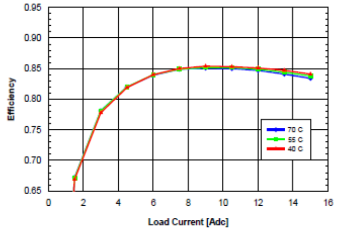
Fig. 1.5V.6: Efficiency vs. load current and ambient temperature for SQ48T/S15015 converter mounted vertically with V_{in} = 48\text{V} and air flowing from pin 3 to pin 1 at a rate of 200LFM (1.0 m/s).
