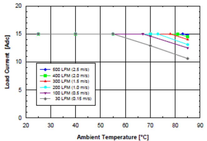
Figure 2.5V.2 Available load current vs. ambient air temperature and airflow rates for SQ48T15025 converter with D height pins mounted horizontally with V_{in} = 48V , air flowing from pin 3 to pin 1, and maximum FET temperature \leq 120^{\circ}C .
