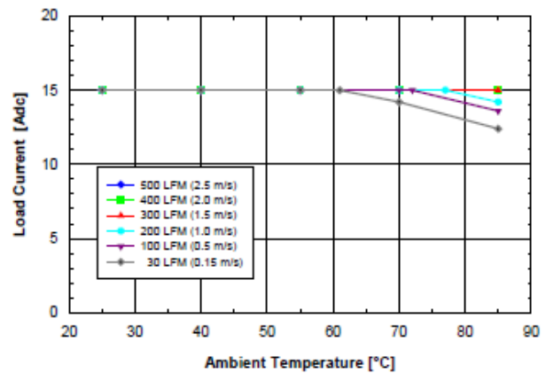
Figure 2.0V.2 Available load current vs. ambient air temperature and airflow rates for SQ48T15020 converter with D height pins mounted horizontally with V_{in} = 48V , air flowing from pin 3 to pin 1, and maximum FET temperature \leq 120^{\circ}C .
