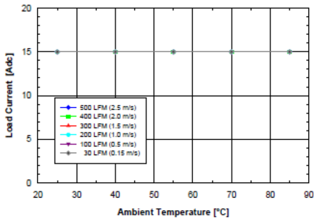
Figure 1.0V.1 Available load current vs. ambient air temperature and airflow rates for SQ48T15010 converter with D height pins mounted vertically with V_{in} = 48V , air flowing from pin 3 to pin 1, and maximum FET temperature \leq 120^{\circ}C .
