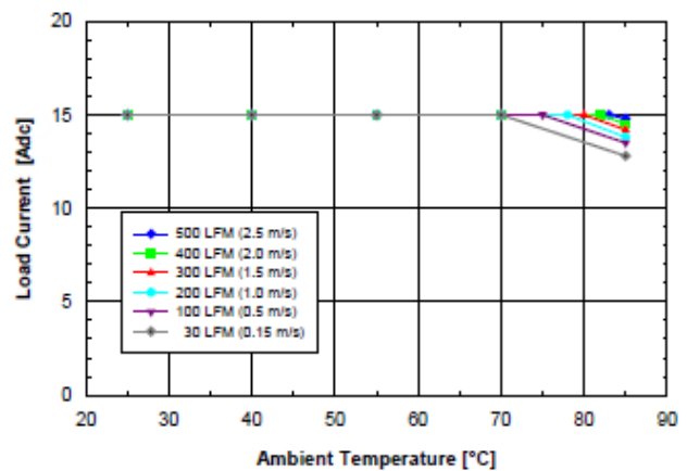
Figure 2.0V.4 Available load current vs. ambient air temperature and airflow rates for SQ48S15020 converter with D height pins mounted horizontally with V_{in} = 48V , air flowing from pin 3 to pin 1, and maximum FET temperature \leq 120^{\circ}C .
