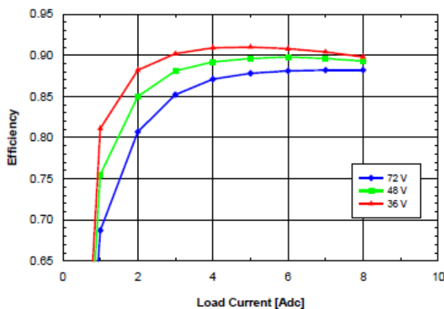
Fig. 6.0V.3: Efficiency vs. load current and input voltage for SQ48T/S08060 converter mounted vertically with air flowing from pin 3 to pin 1 at a rate of 300LFM (1.5 m/s) and T_a = 25^{\circ}C .
