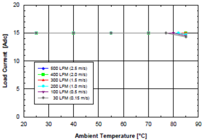
Figure 1.2V.4 Available load current vs. ambient air temperature and airflow rates for SQ48S15012 converter with D height pins mounted horizontally with V_{in} = 48V , air flowing from pin 3 to pin 1, and maximum FET temperature \leq 120^{\circ}C .
