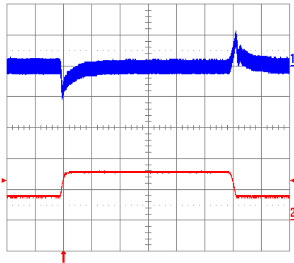
Fig. 2.5V.11: Output voltage response to load current step-change (3.75 A – 7.5 A – 3.75 A) at V_{in} = 48V . Top trace: output voltage (100mV/div.). Bottom trace: load current (5A/div.). Current slew rate: 0.1A/ \mu s . C_o = 1\mu F ceramic. Time scale: 0.2 ms/div.
