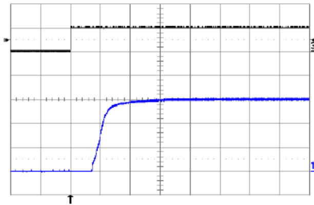
Fig. 6.0V.7: Turn-on transient at full rated load current (resistive) with no output capacitor at V_{in} = 48\text{V} , triggered via ON/OFF pin. Top trace: ON/OFF signal (5V/div.). Bottom trace: output voltage (2V/div.). Time scale: 2ms/div.
