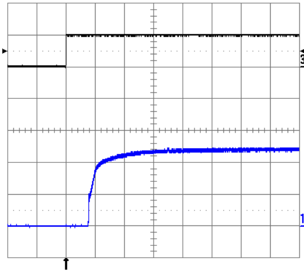
Fig. 1.2V.9: Turn-on transient at full rated load current (resistive) with no output capacitor at V_{in} = 48V , triggered via ON/OFF pin. Top trace: ON/OFF signal 5V/div.). Bottom trace: output voltage (0.5V/div.). Time scale: 2ms/div.
