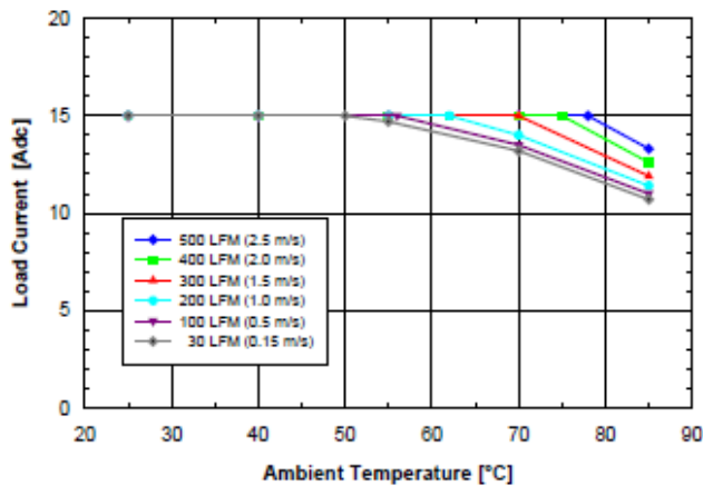
Figure 2.5V.3 Available load current vs. ambient air temperature and airflow rates for SQ48S15025 converter with D height pins mounted vertically with V_{in} = 48V , air flowing from pin 3 to pin 1, and maximum FET temperature \leq 120^{\circ}C .
