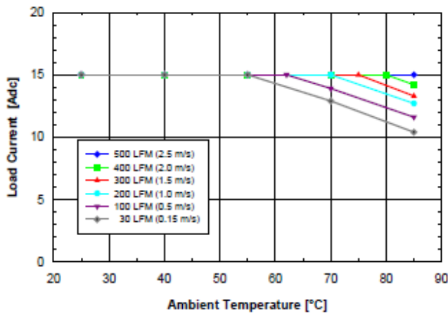
Figure 2.5V.1 Available load current vs. ambient air temperature and airflow rates for SQ48T15025 converter with D height pins mounted vertically with V_{in} = 48V , air flowing from pin 3 to pin 1, and maximum FET temperature \leq 120^{\circ}C .
