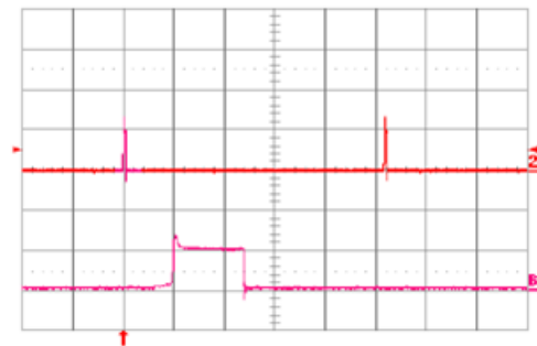
Fig. 1.2V.16: Input reflected ripple current, i_s (10 mA/div.), measured through 10\mu\text{H} at the source at full rated full rated load current and V_{in} = 48\text{V} . Refer to Fig. 1.2V.14 for test setup. Time scale: 1\mu\text{s}/\text{div} .
