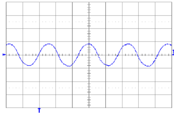
Fig. 12V.11: Output voltage ripple (50 mV/div.) at full rated load current into a resistive load with C_o = 10\mu F tantalum + 1 \mu F ceramic and V_{in} = 48V . Time scale: 1 \mu s/div.
