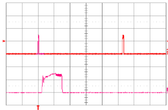
Fig. 8.0V.16: Load current (top trace, 5A/div., 20 ms/div.) into a 10 m\Omega short circuit during restart, at V_{in} = 48V . Bottom trace (5A/div., 1ms/div.) is an expansion of the on-time portion of the top trace.
