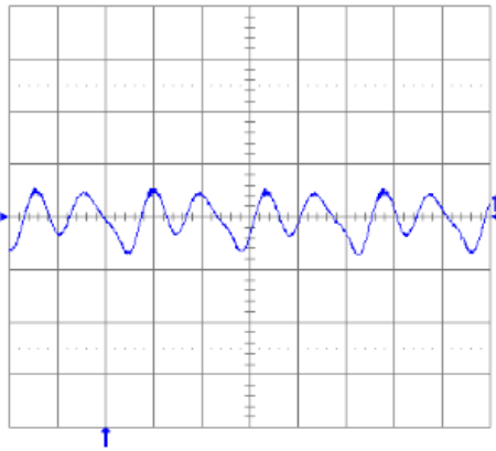
Fig. 1.2V.13: Output voltage ripple (20 mV/div.) at full rated load current into a resistive load with C_o = 10\mu\text{F} tantalum + 1\mu\text{F} ceramic and V_{in} = 48\text{V} . Time scale: 1\mu\text{s}/\text{div} .
