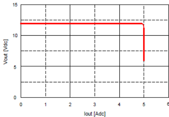
Fig. 12V.15: Output voltage vs. load current showing current limit point and converter shutdown point. Input voltage has almost no effect on current limit characteristic.
