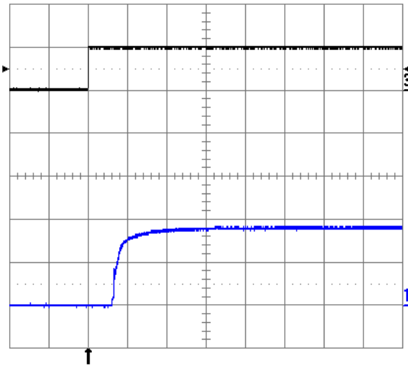
Fig. 1.8V.9: Turn-on transient at full rated load current (resistive) with no output capacitor at V_{in} = 48V , triggered via ON/OFF pin. Top trace: ON/OFF signal (5V/div.). Bottom trace: output voltage (1V/div.). Time scale: 2ms/div.
