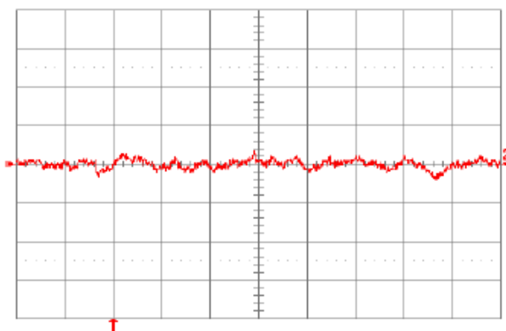
Fig. 5.0V.16: Input reflected ripple current, i_s (10 mA/div.), measured through 10\mu\text{H} at the source at full rated full rated load current and V_{in} = 48\text{V} . Refer to Fig. 5.0V.14 for test setup. Time scale: 1\mu\text{s}/\text{div} .
