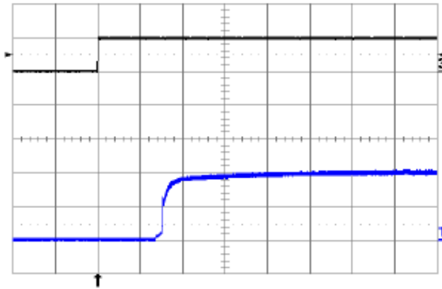
Fig. 1.0V.9: Turn-on transient at full rated load current (resistive) with no output capacitor at V_{in} = 48V , triggered via ON/OFF pin. Top trace: ON/OFF signal 5V/div.). Bottom trace: output voltage (0.5V/div.). Time scale: 2ms/div.
