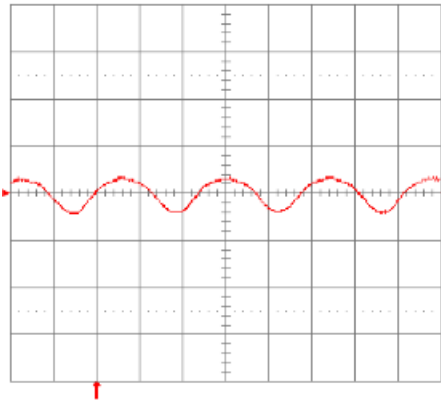
Fig. 1.5V.15: Input reflected ripple current, i_c (100 mA/div.), measured at input terminals at full rated load current and V_{in} = 48\text{V} . Refer to Fig. 1.5V.14 for test setup. Time scale: 1\mu\text{s}/\text{div} .
