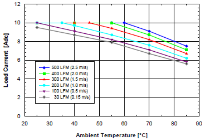
Figure 5.0V.3 Available load current vs. ambient air temperature and airflow rates for SQ48S10050 converter with D height pins mounted vertically with V_{in} = 48V , air flowing from pin 3 to pin 1, and maximum FET temperature \leq 120^{\circ}C .
