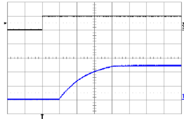
Fig. 12V.8: Turn-on transient at full rated load current (resistive) plus 1,000 \mu\text{F} at V_{in} = 48\text{V} , triggered via ON/OFF pin. Top trace: ON/OFF signal (5V/div.). Bottom trace: output voltage (5V/div.). Time scale: 2ms/div.
