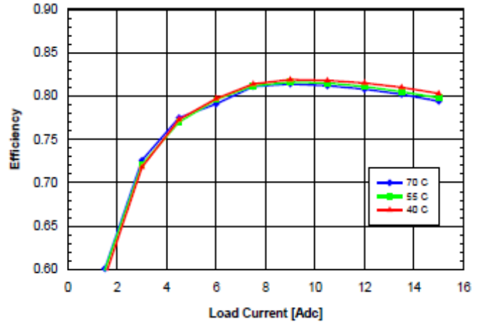
Fig. 1.0V.6: Efficiency vs. load current and ambient temperature for SQ48T/S15010 converter mounted vertically with V_{in} = 48\text{V} and air flowing from pin 3 to pin 1 at a rate of 200LFM (1.0 m/s).
