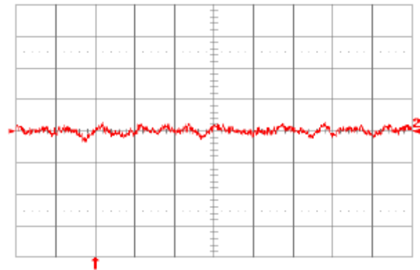
Fig. 1.0V.16: Input reflected ripple current, i_s (10 mA/div.), measured through 10\mu\text{H} at the source at full rated full rated load current and V_{in} = 48\text{V} . Refer to Fig. 1.0V.14 for test setup. Time scale: 1\mu\text{s}/\text{div} .
