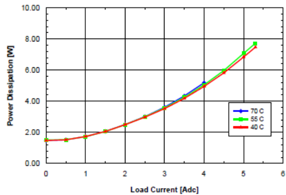
Fig. 8.0V.6: Power dissipation vs. load current and ambient temperature for SQ48T/S05080 converter mounted vertically with V_{in} = 48\text{V} and air flowing from pin 3 to pin 1 at a rate of 200LFM (1.0m/s).
