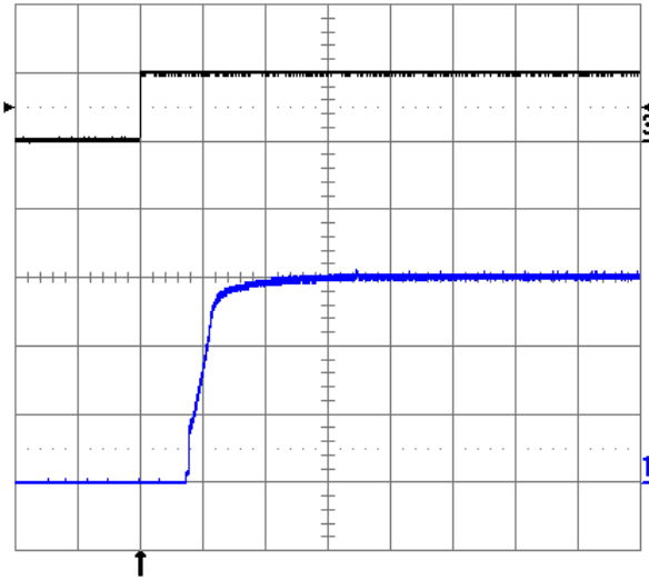
Fig. 1.5V.9: Turn-on transient at full rated load current (resistive) with no output capacitor at V_{in} = 48V , triggered via ON/OFF pin. Top trace: ON/OFF signal (5V/div.). Bottom trace: output voltage (0.5V/div.). Time scale: 2ms/div.
