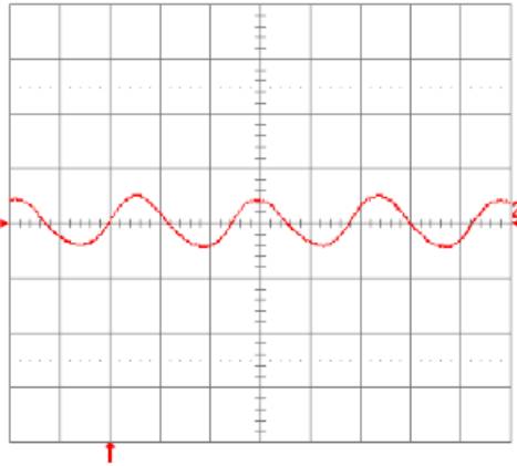
Fig. 3.3V.15: Input reflected ripple current, i_c (100 mA/div.), measured at input terminals at full rated load current and V_{in} = 48\text{V} . Refer to Fig. 3.3V.14 for test setup. Time scale: 1\mu\text{s}/\text{div} .
