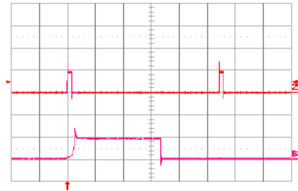
Fig. 1.0V.18: Load current (top trace, 20A/div., 20 ms/div.) into a 10\text{ m}\Omega short circuit during restart, at V_{in} = 48\text{V} . Bottom trace (20A/div., 1ms/div.) is an expansion of the on-time portion of the top trace.
