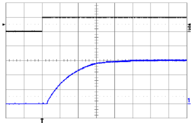
Fig. 6.0V.8: Turn-on transient at full rated load current (resistive) plus 10,000 \mu\text{F} at V_{in} = 48\text{V} , triggered via ON/OFF pin. Top trace: ON/OFF signal (5V/div.). Bottom trace: output voltage (2V/div.). Time scale: 5ms/div.
