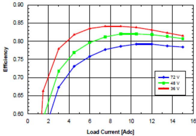
Fig. 1.0V.5: Efficiency vs. load current and input voltage for SQ48T/S15010 converter mounted vertically with air flowing from pin 3 to pin 1 at a rate of 300LFM (1.5 m/s) and T_a = 25^\circ\text{C} .
