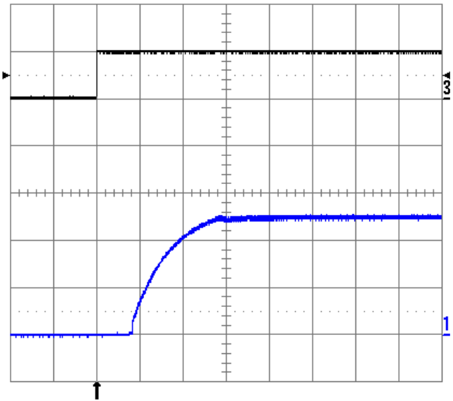
Fig. 2.5V.10: Turn-on transient at full rated load current (resistive) plus 10,000 \mu F at V_{in} = 48V , triggered via ON/OFF pin. Top trace: ON/OFF signal (5V/div.). Bottom trace: output voltage (1V/div.). Time scale: 2ms/div.
