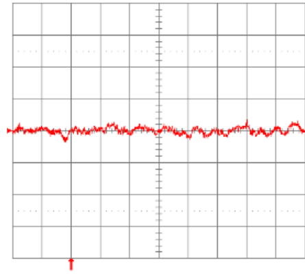
Fig. 1.5V.16: Input reflected ripple current, i_s (10 mA/div.), measured through 10\mu\text{H} at the source at full rated full rated load current and V_{in} = 48\text{V} . Refer to Fig. 1.5V.14 for test setup. Time scale: 1\mu\text{s}/\text{div} .
