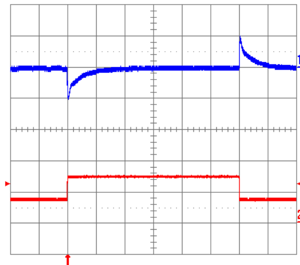
Fig. 3.3V.12: Output voltage response to load current step-change (3.75 A - 7.5 A - 3.75 A) at V_{in} = 48V . Top trace: output voltage (100 mV/div.). Bottom trace: load current (5A/div.). Current slew rate: 5 A/ \mu s . C_o = 450\mu F tantalum + 1 \mu F ceramic. Time scale: 0.2 ms/div.
