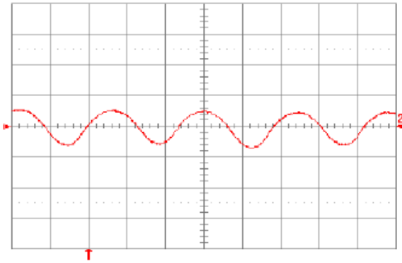
Fig. 8.0V.13: Input reflected ripple current, i_c (100 mA/div.), measured at input terminals at full rated load current and V_{in} = 48V . Refer to Fig. 8.0V.14 for test setup. Time scale: 1\mu s/div .
