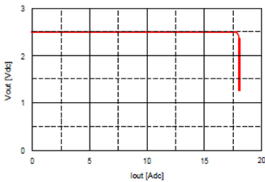
Fig. 2.5V.17: Output voltage vs. load current showing current limit point and converter shutdown point. Input voltage has almost no effect on current limit characteristic.
