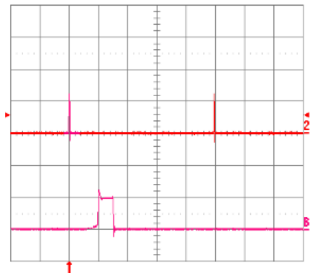
Fig. 2.5V.18: Load current (top trace, 20A/div., 20 ms/div.) into a 10\text{m}\Omega short circuit during restart, at V_{in} = 48\text{V} . Bottom trace (20A/div., 1ms/div.) is an expansion of the on-time portion of the top trace.
