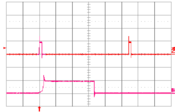
Fig. 1.0V.18: Load current (top trace, 20\text{A}/\text{div} ., 20\text{ms}/\text{div} .) into a 10\text{m}\Omega short circuit during restart, at V_{in} = 48\text{V} . Bottom trace ( 20\text{A}/\text{div} ., 1\text{ms}/\text{div} .) is an expansion of the on-time portion of the top trace.
