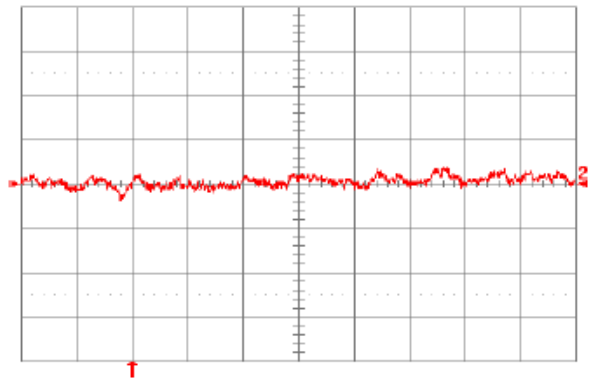
Fig. 12V.14: Input reflected ripple current, i_s (100 mA/div.), measured at input terminals at full rated full rated load current and V_{in} = 48V . Refer to Fig. 12V.14 for test setup. Time scale: 1\mu s/div .
