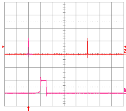
Fig. 2.5V.18: Load current (top trace, 20\text{A}/\text{div} ., 20\text{ms}/\text{div} .) into a 10\text{m}\Omega short circuit during restart, at V_{in} = 48\text{V} . Bottom trace ( 20\text{A}/\text{div} ., 1\text{ms}/\text{div} .) is an expansion of the on-time portion of the top trace.
