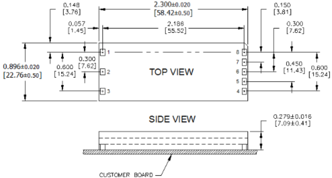
SQ48T Pinout (Through-hole)
