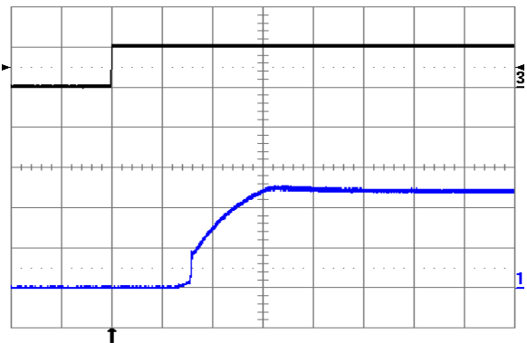
Fig. 1.2V.10: Turn-on transient at full rated load current (resistive) plus 10,000 µF at V in = 24V, triggered via ON/OFF pin. Top trace: ON/OFF signal (5 V/div.). Bottom trace: output voltage (0.5 V/div.). Time scale: 1 ms/div.
