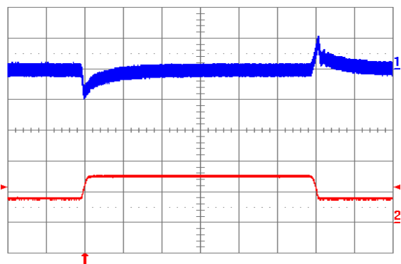
Fig. 2.5V.11: Output voltage response to load current step-change (3.75 A – 7.5 A – 3.75 A) at V in = 24V. Top trace: output voltage (100 mV/div.). Bottom trace: load current (5 A/div.). Current slew rate: 0.1 A/µs. C o = 1 µF ceramic. Time scale: 0.2 ms/div.
