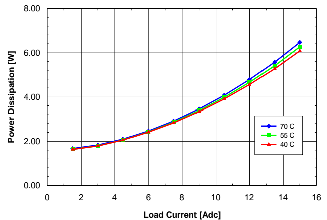
Fig. 2.5V.8: Power dissipation vs. load current and ambient temperature for SQ24T/S15025 converter mounted vertically with V in = 24V and air flowing from pin 3 to pin 1 at a rate of 200 LFM (1.0 m/s).
