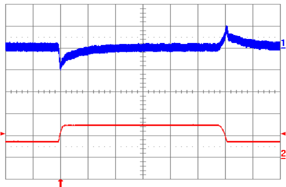
Fig. 3.3V.11: Output voltage response to load current step-change (3.75A – 7.5A – 3.75A) at V in = 24V. Top trace: output voltage (100 mV/div.). Bottom trace: load current (5 A/div.). Current slew rate: 0.1 A/µs. C o = 1 µF ceramic. Time scale: 0.2 ms/div.
