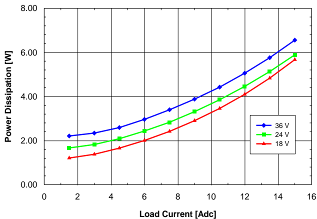
Fig. 2.5V.7: Power dissipation vs. load current and input voltage for SQ24T/S15025 converter mounted vertically with air flowing from pin 3 to pin 1 at a rate of 300 LFM (1.5 m/s) and T a = 25°C.
