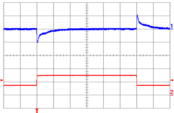
Fig. 3.3V.12: Output voltage response to load current step-change (3.75A – 7.5A – 3.75A) at V in = 24V. Top trace: output voltage (100 mV/div.). Bottom trace: load current (5 A/div.). Current slew rate: 5 A/µs. C o = 450 µF tantalum + 1 µF ceramic. Time scale: 0.2 ms/div.
