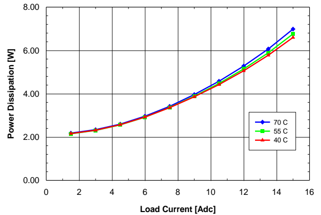
Fig. 3.3V.8: Power dissipation vs. load current and ambient temperature for SQ24T/S15033 converter mounted vertically with V in = 24V and air flowing from pin 3 to pin 1 at a rate of 200 LFM (1.0 m/s).
