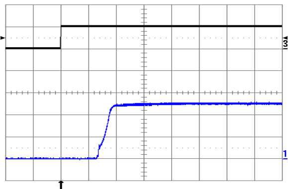
Fig. 2.5V.9: Turn-on transient at full rated load current (resistive) with no output capacitor at V in = 24V, triggered via ON/OFF pin. Top trace: ON/OFF signal (5 V/div.). Bottom trace: output voltage (1 V/div.). Time scale: 1 ms/div.
