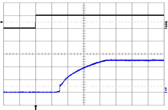
Fig. 2.5V.10: Turn-on transient at full rated load current (resistive) plus 10,000 µF at V in = 24V, triggered via ON/OFF pin. Top trace: ON/OFF signal (5 V/div.). Bottom trace: output voltage (1 V/div.). Time scale: 1 ms/div.
