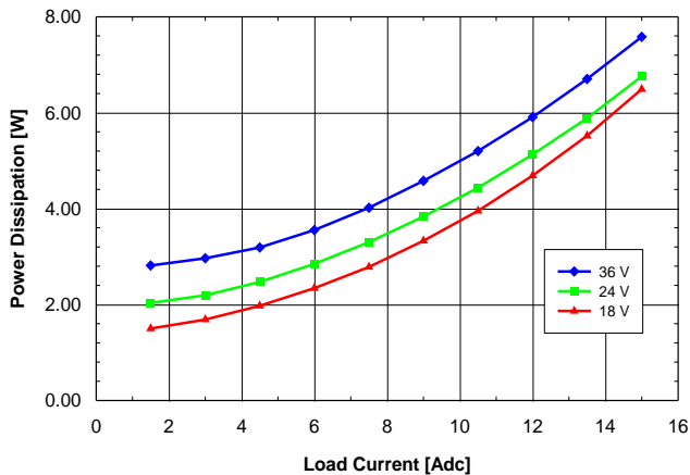
Fig. 3.3V.7: Power dissipation vs. load current and input voltage for SQ24T/S15033 converter mounted vertically with air flowing from pin 3 to pin 1 at a rate of 300 LFM (1.5 m/s) and T a = 25°C.
