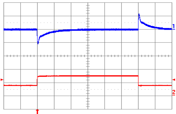
Fig. 1.2V.12: Output voltage response to load current step-change (3.75 A – 7.5 A – 3.75 A) at V in = 24V. Top trace: output voltage (100 mV/div.). Bottom trace: load current (5 A/div.). Current slew rate: 5 A/µs. Co = 450 µF tantalum + 1 µF ceramic. Time scale: 0.2 ms/div.
