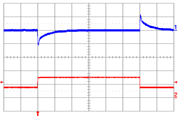
Fig. 2.5V.12: Output voltage response to load current step-change (3.75 A – 7.5 A – 3.75 A) at V in = 24V. Top trace: output voltage (100 mV/div.). Bottom trace: load current (5 A/div.). Current slew rate: 5 A/µs. C o = 450 µF tantalum + 1 µF ceramic. Time scale: 0.2 ms/div.
