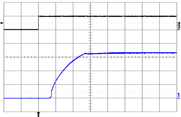
Fig. 3.3V.10: Turn-on transient at full rated load current (resistive) plus 10,000 µF at V in = 24V, triggered via ON/OFF pin. Top trace: ON/OFF signal (5 V/div.). Bottom trace: output voltage (1 V/div.). Time scale: 2 ms/div.
