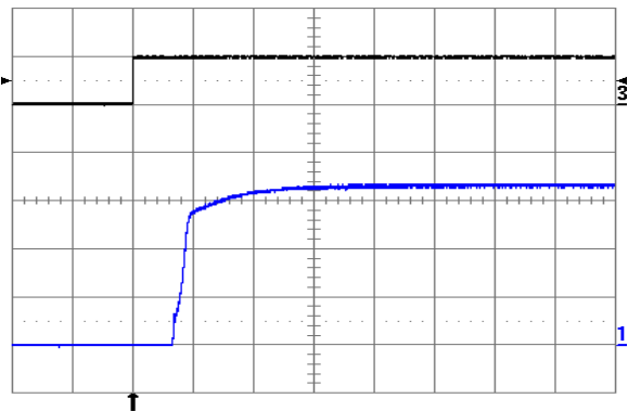
Fig. 3.3V.9: Turn-on transient at full rated load current (resistive) with no output capacitor at V in = 24V, triggered via ON/OFF pin. Top trace: ON/OFF signal (5 V/div.). Bottom trace: output voltage (1 V/div.). Time scale: 2 ms/div.
