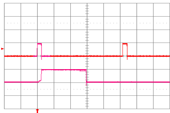
Fig. 1.2V.18: Load current (top trace, 20 A/div., 20 ms/div.) into a 10 \text{ m}\Omega short circuit during restart, at V_{in} = 24 \text{ V} . Bottom trace (20 A/div., 2 ms/div.) is an expansion of the on-time portion of the top trace.
