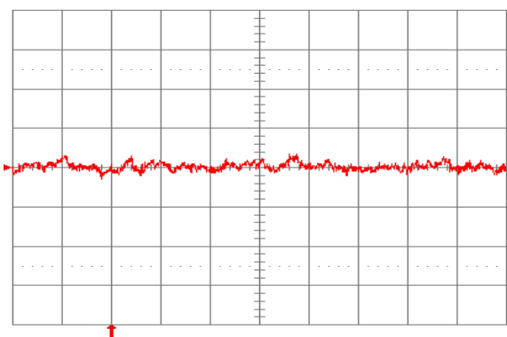
Fig. 1.2V.16: Input reflected ripple current, i_s (10 mA/div.), measured through 10 \mu\text{H} at the source at full rated load current and V_{in} = 24 \text{ V} . Refer to Fig. 1.2V.14 for test setup. Time scale: 1 \mu\text{s}/\text{div} .
