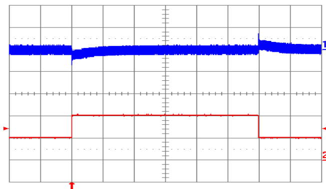
Fig. 12V.12: Output voltage response to load current step-change (1 A – 2 A – 1 A) at V_{in} = 24\text{V} . Top trace: output voltage (200 mV/div.). Bottom trace: load current (1 A/div.). Current slew rate: 5 A/µs. C_o = 1\text{ µF} ceramic. Time scale: 0.5 ms/div.
