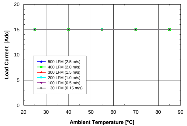
Fig. 1.0V.4: Available load current vs. ambient air temperature and airflow rates for SQ24S15010 converter mounted horizontally with V_{in} = 24V , air flowing from pin 3 to pin 1 and maximum FET temperature \leq 120^{\circ}C .
