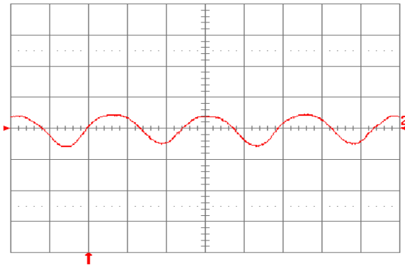
Fig. 1.8V.15: Input reflected ripple current, i_c (100 mA/div.), measured at input terminals at full rated load current and V_{in} = 24\text{V} . Refer to Fig. 1.8V.14 for test setup. Time scale: 1 \mu\text{s}/\text{div} .
