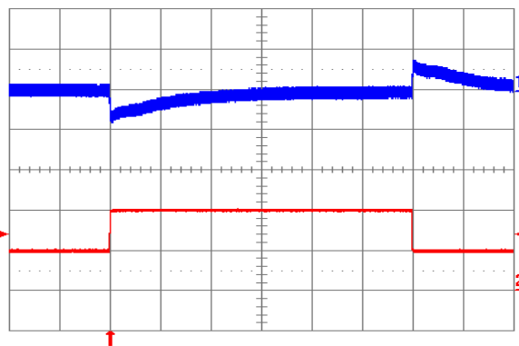
Fig. 6.0V.12: Output voltage response to load current step-change (2A - 4A - 2A) at V_{in} = 24\text{V} . Top trace: output voltage (100 mV/div.). Bottom trace: load current (2 A/div.). Current slew rate: 5 A/µs. C_o = 450 \mu\text{F} tantalum + 1 µF ceramic. Time scale: 0.2 ms/div.
