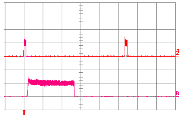
Fig. 12V.18: Load current (top trace, 5\ \text{A}/\text{div} ., 20\ \text{ms}/\text{div} .) into a 10\ \text{m}\Omega short circuit during restart, at V_{in} = 24\ \text{V} . Bottom trace ( 5\ \text{A}/\text{div} ., 1\ \text{ms}/\text{div} .) is an expansion of the on-time portion of the top trace.
