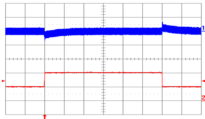
Fig. 12V.11: Output voltage response to load current step-change (1 A – 2 A – 1 A) at V_{in} = 24\text{V} . Top trace: output voltage (200 mV/div.). Bottom trace: load current (1 A/div.). Current slew rate: 0.1 A/µs. C_o = 1\text{ µF} ceramic. Time scale: 0.5 ms/div.
