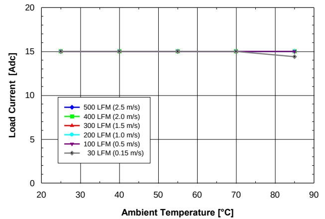
Fig. 1.8V.4: Available load current vs. ambient air temperature and airflow rates for SQ24S15018 converter mounted horizontally with V_{in} = 24V , air flowing from pin 3 to pin 1 and maximum FET temperature \leq 120^{\circ}C .
