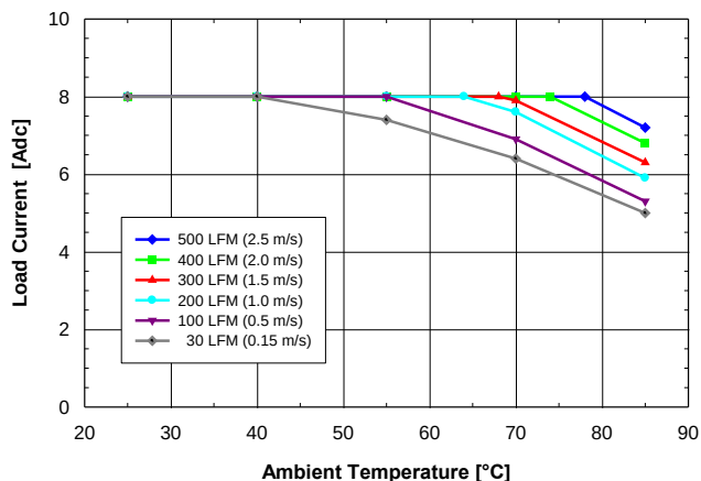
Fig. 6.0V.1: Available load current vs. ambient air temperature and airflow rates for SQ24T08060 converter with B height pins mounted vertically with V_{in} = 24V , air flowing from pin 3 to pin 1 and maximum FET temperature \leq 120^{\circ}C .
