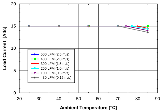
Fig. 1.8V.3: Available load current vs. ambient air temperature and airflow rates for SQ24S15018 converter mounted vertically with V_{in} = 24V , air flowing from pin 3 to pin 1 and maximum FET temperature \leq 120^{\circ}C .
