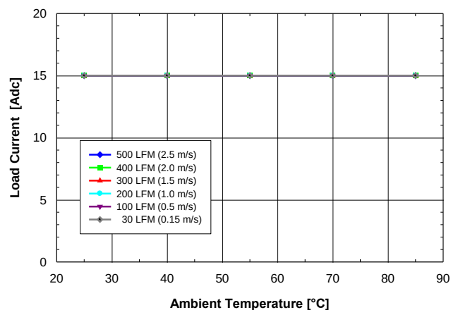
Fig. 1.2V.4: Available load current vs. ambient temperature and airflow rates for SQ24S15012 converter mounted horizontally with V_{in} = 24V , air flowing from pin 3 to pin 1 and maximum FET temperature \leq 120^{\circ}C .
