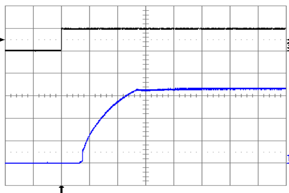
Fig. 3.3V.10: Turn-on transient at full rated load current (resistive) plus 10,000 µF at V_{in} = 24\text{V} , triggered via ON/OFF pin. Top trace: ON/OFF signal (5 V/div.). Bottom trace: output voltage (1 V/div.). Time scale: 2 ms/div.
