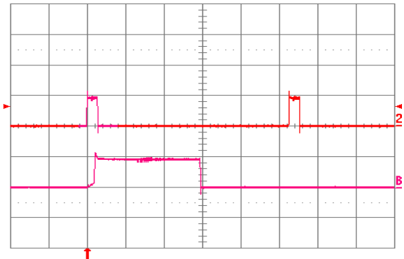
Fig. 1.8V.18: Load current (top trace, 20 A/div., 20 ms/div.) into a 10 \text{ m}\Omega short circuit during restart, at V_{in} = 24\text{V} . Bottom trace (20 A/div., 2 ms/div.) is an expansion of the on-time portion of the top trace.
