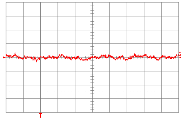
Fig. 2.0V.16: Input reflected ripple current, i_s (10 mA/div.), measured through 10 \mu\text{H} at the source at full rated load current and V_{in} = 24 \text{ V} . Refer to Fig. 2.0V.14 for test setup. Time scale: 1 \mu\text{s}/\text{div.}
