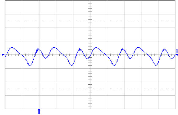
Fig. 1.0V.13: Output voltage ripple (20 mV/div.) at full rated load current into a resistive load with C_o = 10 \mu\text{F} tantalum + 1\mu\text{F} ceramic and V_{in} = 24 \text{V} . Time scale: 1 \mu\text{s}/\text{div} .
