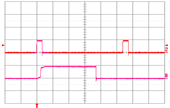
Fig. 1.0V.18: Load current (top trace, 20 A/div., 20 ms/div.) into a 10 \text{m}\Omega short circuit during restart, at V_{in} = 24\text{V} . Bottom trace (20 A/div., 2 ms/div.) is an expansion of the on-time portion of the top trace.
