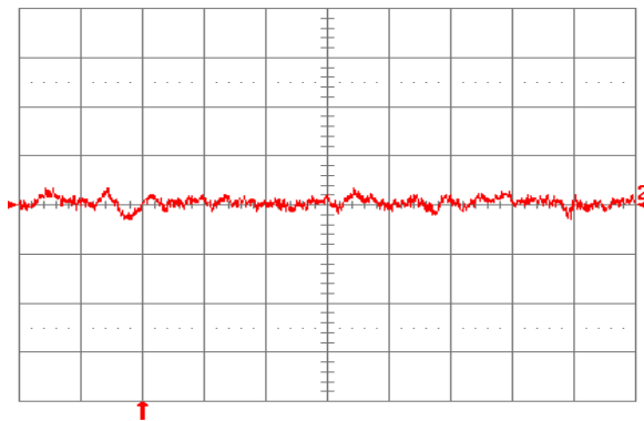
Fig. 2.5V.16: Input reflected ripple current, i_s (10 mA/div.), measured through 10 \mu\text{H} at the source at full rated load current and V_{in} = 24 \text{ V} . Refer to Fig. 2.5V.14 for test setup. Time scale: 1 \mu\text{s}/\text{div} .
