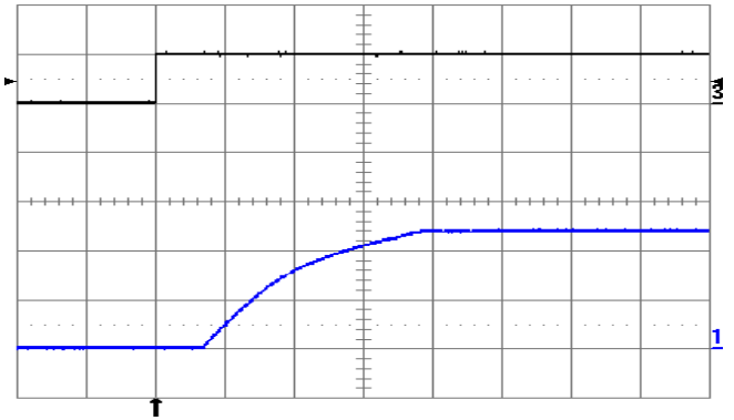
Fig. 12V.10: Turn-on transient at full rated load current (resistive) plus 1,000 \mu\text{F} at V_{in} = 24\text{V} , triggered via ON/OFF pin. Top trace: ON/OFF signal (5 V/div.). Bottom trace: output voltage (5 V/div.). Time scale: 2 ms/div.
