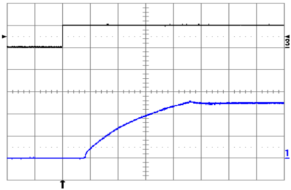
Fig. 5.0V.10: Turn-on transient at full rated load current (resistive) plus 10,000 µF at Vin = 24V, triggered via ON/OFF pin. Top trace: ON/OFF signal (5 V/div.). Bottom trace: output voltage (2 V/div.). Time scale: 2 ms/div.
