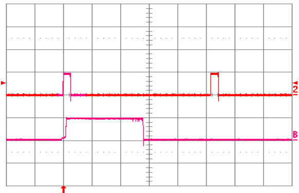
Fig. 1.5V.18: Load current (top trace, 20 A/div., 20 ms/div.) into a 10 \text{ m}\Omega short circuit during restart, at V_{in} = 24\text{V} . Bottom trace (20 A/div., 2 ms/div.) is an expansion of the on-time portion of the top trace.
