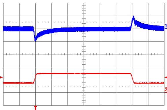
Fig. 1.5V.11: Output voltage response to load current step-change (3.75 A – 7.5 A – 3.75 A) at V in = 24V. Top trace: output voltage (100 mV/div.). Bottom trace: load current (5 A/div.). Current slew rate: 0.1 A/µs. C o = 1 µF ceramic. Time scale: 0.2 ms/div.
