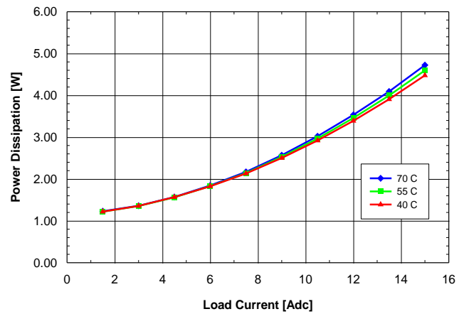
Fig. 1.5V.8: Power dissipation vs. load current and ambient temperature for SQ24T/S15015 converter mounted vertically with V in = 24V and air flowing from pin 3 to pin 1 at a rate of 200 LFM (1.0 m/s).
