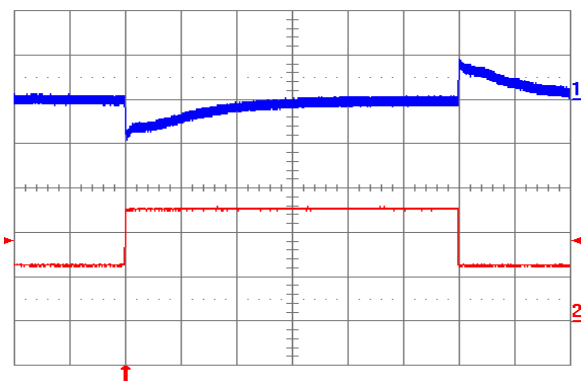
Fig. 5.0V.12: Output voltage response to load current step-change (2.5A - 5A - 2.5A) at Vin = 24V. Top trace: output voltage (100 mV/div.). Bottom trace: load current (2 A/div.). Current slew rate: 5 A/µs. Co = 450 µF tantalum + 1 µF ceramic. Time scale: 0.2 ms/div.
