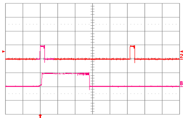
Fig. 2.0V.18: Load current (top trace, 20 A/div., 20 ms/div.) into a 10 \text{m}\Omega short circuit during restart, at V_{in} = 24 \text{ V} . Bottom trace (20 A/div., 2 ms/div.) is an expansion of the on-time portion of the top trace.
