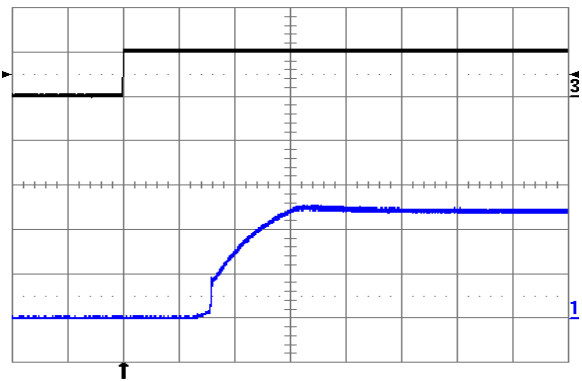
Fig. 1.2V.10: Turn-on transient at full rated load current (resistive) plus 10,000 µF at V in = 24V, triggered via ON/OFF pin. Top trace: ON/OFF signal (5 V/div.). Bottom trace: output voltage (0.5 V/div.). Time scale: 1 ms/div.
