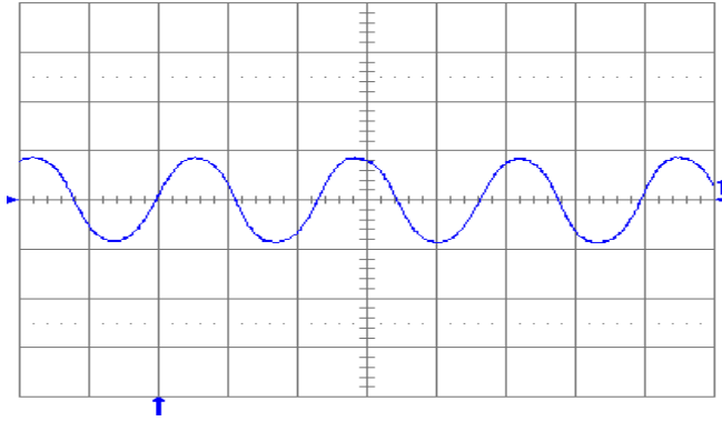
Fig. 12V.13: Output voltage ripple (50 mV/div.) at full rated load current into a resistive load with C_o = 10 \mu\text{F} tantalum + 1 \mu\text{F} ceramic and V_{in} = 24 \text{ V} . Time scale: 1 \mu\text{s}/\text{div} .
