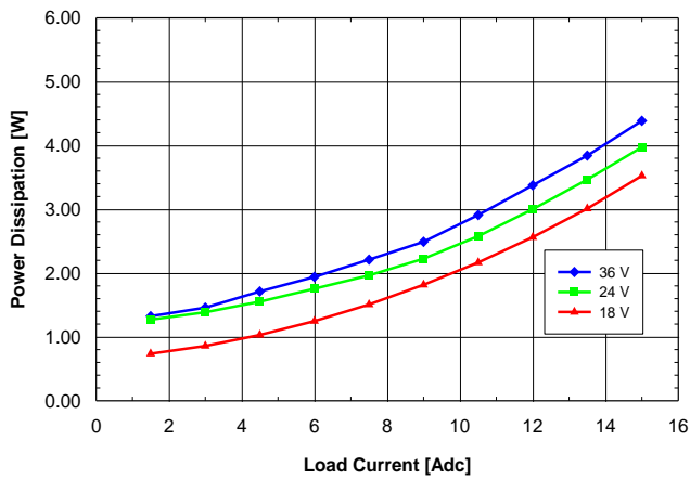
Fig. 1.0V.7: Power dissipation vs. load current and input voltage for SQ24T/S15010 converter mounted vertically with air flowing from pin 3 to pin 1 at a rate of 300 LFM (1.5 m/s) and T a = 25°C.
