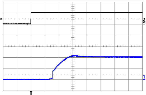
Fig. 1.0V.10: Turn-on transient at full rated load current (resistive) plus 10,000µF at V in = 24V, triggered via ON/OFF pin. Top trace: ON/OFF signal (5 V/div.). Bottom trace: output voltage (0.5 V/div.). Time scale: 1 ms/div.
