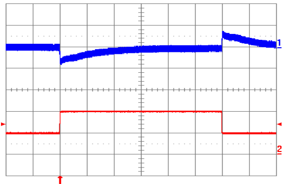
Fig. 6.0V.12: Output voltage response to load current step-change (2A - 4A - 2A) at V_{in} = 24\text{V} . Top trace: output voltage (100mV/div.). Bottom trace: load current (2A/div.). Current slew rate: 5 A/ \mu\text{s} . C_o = 450\ \mu\text{F} tantalum + 1 \mu\text{F} ceramic. Time scale: 0.2 ms/div.
