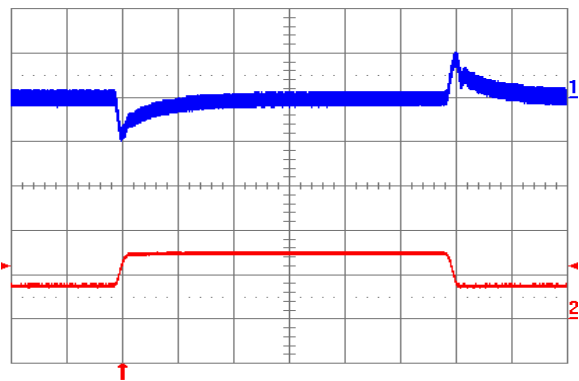
Fig. 1.2V.11: Output voltage response to load current step-change (3.75 A – 7.5 A – 3.75 A) at V in = 24V. Top trace: output voltage (100 mV/div.). Bottom trace: load current (5 A/div.). Current slew rate: 0.1 A/µs. Co = 1 µF ceramic. Time scale: 0.2 ms/div.
