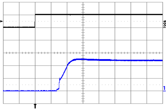
Fig. 1.2V.9: Turn-on transient at full rated load current (resistive) with no output capacitor at V in = 24V, triggered via ON/OFF pin. Top trace: ON/OFF signal (5 V/div.). Bottom trace: output voltage (0.5 V/div.). Time scale: 1 ms/div.
