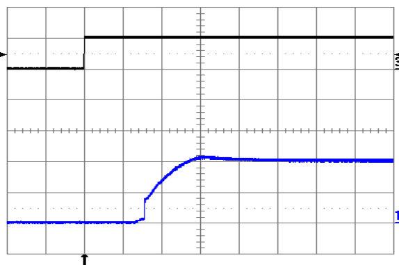
Fig. 1.0V.10: Turn-on transient at full rated load current (resistive) plus 10,000µF at V in = 24V, triggered via ON/OFF pin. Top trace: ON/OFF signal (5 V/div.). Bottom trace: output voltage (0.5 V/div.). Time scale: 1 ms/div.
