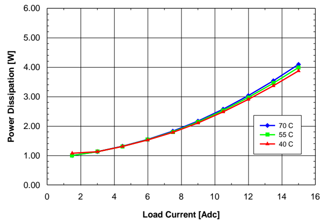
Fig. 1.0V.8: Power dissipation vs. load current and ambient temperature for SQ24T/S15010 converter mounted vertically with V in = 24V and air flowing from pin 3 to pin 1 at a rate of 200 LFM (1.0 m/s).
