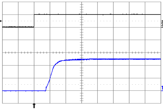
Fig. 5.0V.9: Turn-on transient at full rated load current (resistive) with no output capacitor at Vin = 24V, triggered via ON/OFF pin. Top trace: ON/OFF signal (5 V/div.). Bottom trace: output voltage (2 V/div.). Time scale: 2 ms/div.
