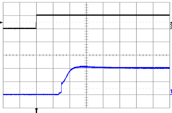
Fig. 1.0V.9: Turn-on transient at full rated load current (resistive) with no output capacitor at V in = 24V, triggered via ON/OFF pin. Top trace: ON/OFF signal (5 V/div.). Bottom trace: output voltage (0.5 V/div.). Time scale: 1 ms/div.
