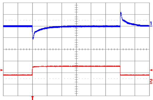
Fig. 1.5V.12: Output voltage response to load current step-change (3.75 A – 7.5 A – 3.75 A) at V in = 24V. Top trace: output voltage (100 mV/div.). Bottom trace: load current (5 A/div.). Current slew rate: 5 A/µs. C o = 450 µF tantalum + 1 µF ceramic. Time scale: 0.2 ms/div.
