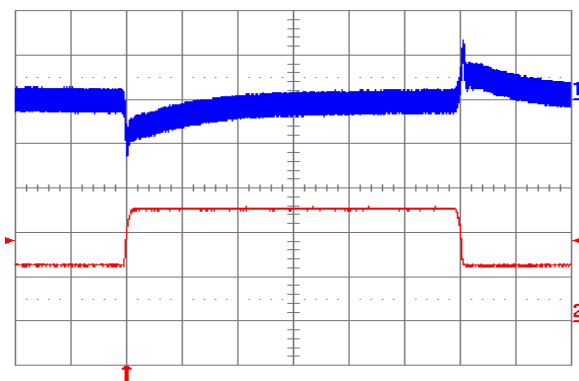
Fig. 5.0V.11: Output voltage response to load current step-change (2.5A - 5A - 2.5A) at Vin = 24V. Top trace: output voltage (100 mV/div.). Bottom trace: load current (2 A/div.). Current slew rate: 0.1 A/µs. Co = 1 µF ceramic. Time scale: 0.2 ms/div.
