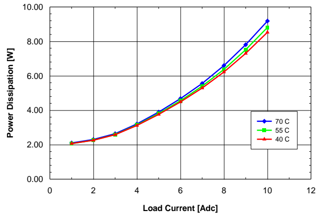
Fig. 5.0V.8: Power dissipation vs. load current and ambient temperature for SQ24T/S10050 converter mounted vertically with Vin = 24V and air flowing from pin 3 to pin 1 at a rate of 200 LFM (1.0 m/s).
