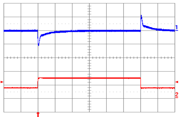
Fig. 1.0V.12: Output voltage response to load current step-change (3.75 A – 7.5 A – 3.75 A) at V in = 24V. Top trace: output voltage (100 mV/div.). Bottom trace: load current (5 A/div.). Current slew rate: 5 A/µs. C o = 450 µF tantalum + 1 µF ceramic. Time scale: 0.2 ms/div.
