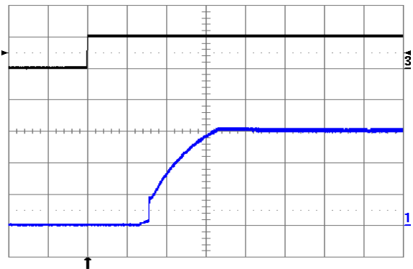
Fig. 1.5V.10: Turn-on transient at full rated load current (resistive) plus 10,000 µF at V in = 24V, triggered via ON/OFF pin. Top trace: ON/OFF signal (5 V/div.). Bottom trace: output voltage (0.5 V/div.). Time scale: 1 ms/div.
