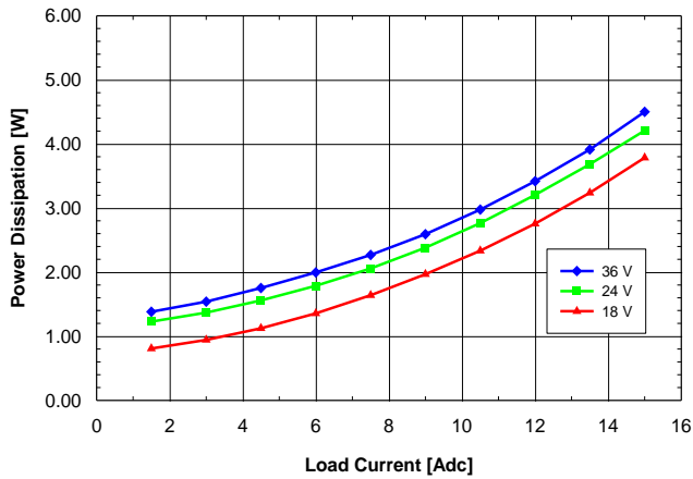
Fig. 1.2V.7: Power dissipation vs. load current and input voltage for SQ24T/S15012 converter mounted vertically with air flowing from pin 3 to pin 1 at a rate of 300 LFM (1.5 m/s) and T a = 25°C.
