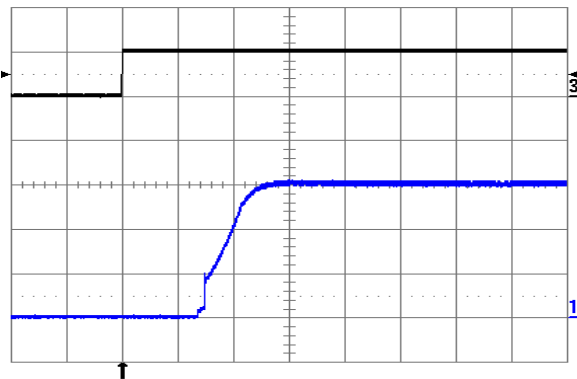
Fig. 1.5V.9: Turn-on transient at full rated load current (resistive) with no output capacitor at V in = 24V, triggered via ON/OFF pin. Top trace: ON/OFF signal (5 V/div.). Bottom trace: output voltage (0.5 V/div.). Time scale: 1 ms/div.
