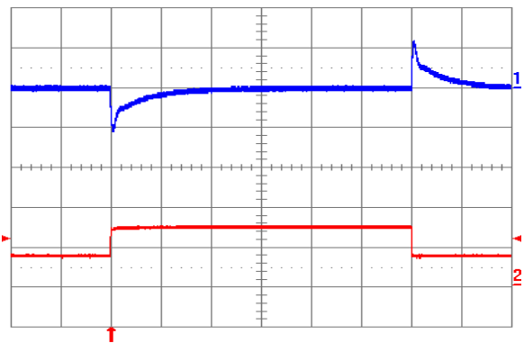
Fig. 1.2V.12: Output voltage response to load current step-change (3.75 A – 7.5 A – 3.75 A) at V in = 24V. Top trace: output voltage (100 mV/div.). Bottom trace: load current (5 A/div.). Current slew rate: 5 A/µs. Co = 450 µF tantalum + 1 µF ceramic. Time scale: 0.2 ms/div.
