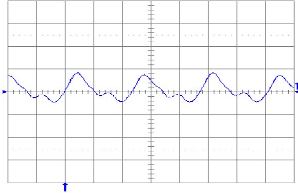
Fig. 3.3V.13: Output voltage ripple (20 mV/div.) at full rated load current into a resistive load with C_o = 10 \mu\text{F} tantalum + 1\mu\text{F} ceramic and V_{in} = 24 \text{ V} . Time scale: 1 \mu\text{s}/\text{div} .
