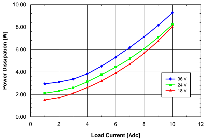
Fig. 5.0V.7: Power dissipation vs. load current and input voltage for SQ24T/S10050 converter mounted vertically with air flowing from pin 3 to pin 1 at a rate of 300 LFM (1.5 m/s) and Ta = 25°C..
