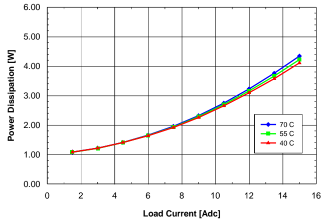
Fig. 1.2V.8: Power dissipation vs. load current and ambient temperature for SQ24T/S15012 converter mounted vertically with V in = 24V and air flowing from pin 3 to pin 1 at a rate of 200 LFM (1.0 m/s).
