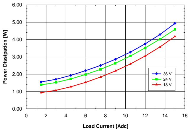
Fig. 1.5V.7: Power dissipation vs. load current and input voltage for SQ24T/S15015 converter mounted vertically with air flowing from pin 3 to pin 1 at a rate of 300 LFM (1.5 m/s) and T a = 25°C.
