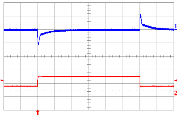
Fig. 1.0V.12: Output voltage response to load current step-change (3.75 A – 7.5 A – 3.75 A) at V in = 24V. Top trace: output voltage (100 mV/div.). Bottom trace: load current (5 A/div.). Current slew rate: 5 A/µs. C o = 450 µF tantalum + 1 µF ceramic. Time scale: 0.2 ms/div.
