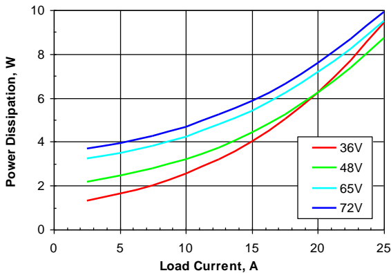
Figure 3. Power dissipation vs. load current and input voltage for SSQE48T25033 converter mounted vertically with air flowing from pin 1 to pin 3 at a rate of 300 LFM (1.5 m/s) and T_a = 25^\circ\text{C} .
