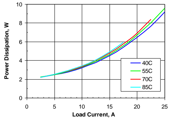
Figure 4. Power dissipation vs. load current and ambient temperature for SSQE48T25033 converter mounted vertically with V_{in} = 48\text{ V} and air flowing from pin 1 to pin 3 at a rate of 200 LFM (1.0 m/s).
