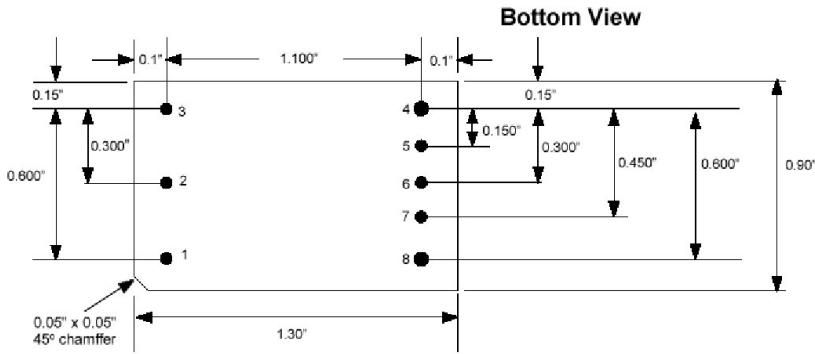
SSQE48T Pinout (Through-hole)
