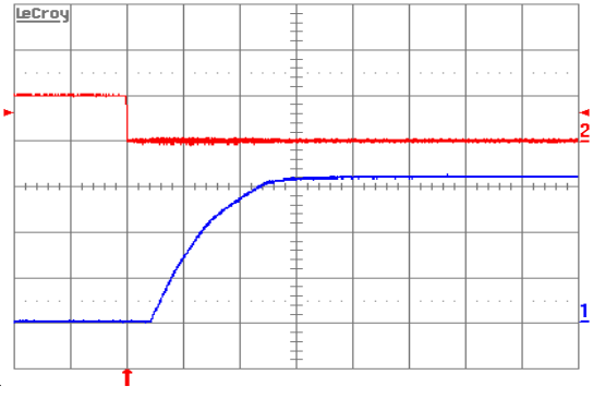
Figure 6. Turn-on transient at full rated load current (resistive) plus 20,000 \mu\text{F} at V_{in} = 48\text{ V} , triggered via ON/OFF pin. Top trace: ON/OFF signal (5 V/div.). Bottom trace: Output voltage (1 V/div.). Time scale: 2 ms/div.
