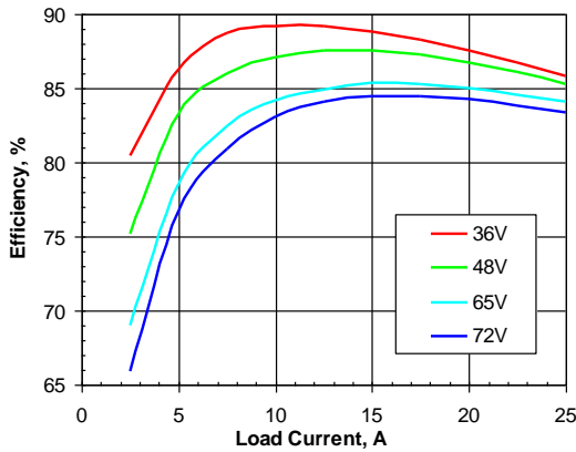
Figure 1. Efficiency vs. load current and input voltage for SSQE48T25033 converter mounted vertically with air flowing from pin 1 to pin 3 at a rate of 300 LFM (1.5 m/s) and T_a = 25^\circ\text{C} .
