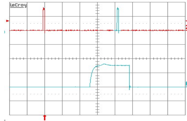
Figure 14. Load current (top trace, 20 A/div., 50 ms/div.) into a 10\ \text{m} short circuit during restart, at V_{in} = 48\ \text{V} . Bottom trace (20 A/div., 2 ms/div.) is an expansion of the on-time portion of the top trace
