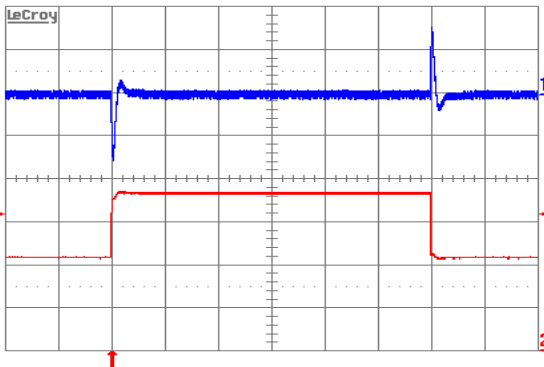
Figure 8. Output voltage response to load current step (12.5 A–18.75 A–12.5 A) at V_{in} = 48\text{ V} . Top trace: output voltage (100 mV/div.). Bottom trace: load current (5 A/div.). Current slew rate: 5 A/ \mu\text{s} . C_o = 470\text{ }\mu\text{F} POS + 1 \mu\text{F} ceramic. Time scale: 0.2 ms/div.
