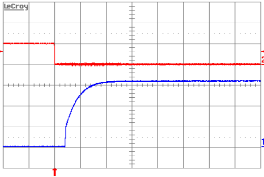
Figure 5. Turn-on transient at full rated load current (resistive) with no output capacitor at V_{in} = 48\text{ V} , triggered via ON/OFF pin. Top trace: ON/OFF signal (5 V/div.). Bottom trace: Output voltage (1.0 V/div.). Time scale: 2 ms/div.
