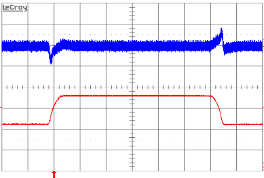
Figure 7. Output voltage response to load current step (12.5 A–18.75 A–12.5 A) at V_{in} = 48\text{ V} . Top trace: output voltage (50 mV/div.). Bottom trace: load current (5 A/div.). Current slew rate: 0.1 A/ \mu\text{s} . C_o = 1\text{ }\mu\text{F} ceramic + 10 \mu\text{F} tantalum. Time scale: 0.2 ms/div.
