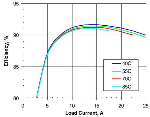
Figure 2. Efficiency vs. load current and ambient temperature for SSQE48T25033 converter mounted vertically with V_{in}=48\text{V} and air flowing from pin 1 to pin 3 at a rate of 200 LFM (1.0m/s).
