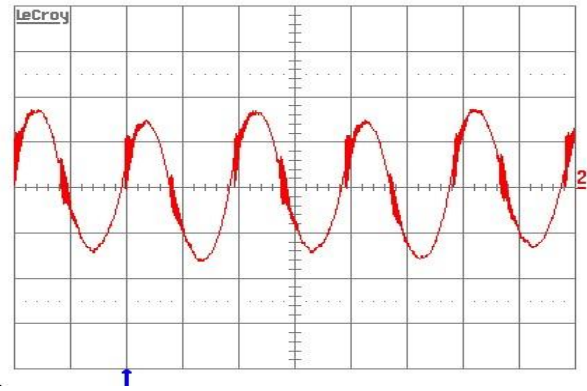
Figure 13. Input reflected ripple-current, i_C (50 mA/div.), measured at input terminals at full rated load current and V_{in} = 48\ \text{V} . Refer to Figure 11 for test setup. Time scale: 1\ \mu\text{s}/\text{div} .
