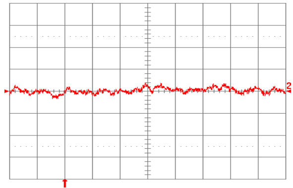
Fig. 1.2V.10: Input reflected ripple current, i_s (10 mA/div.), measured through 10\ \mu\text{H} at the source at full rated load current and V_{in} = 48\ \text{V} . Refer to Fig. 1.2V.8 for test setup. Time scale: 1\ \mu\text{s}/\text{div} .
