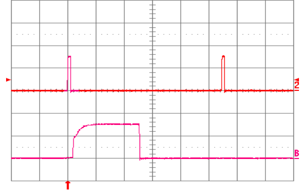
Fig. 2.0V.12: Load current (top trace, 20 A/div., 20 ms/div.) in- to a 10 mΩ short circuit during restart, at Vin = 48 V. Bottom trace (20 A/div., 1 ms/div.) is an expansion of the on-time portion of the top trace.
