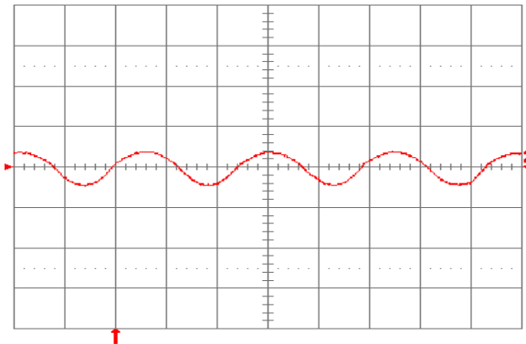
Fig. 2.0V.9: Input reflected ripple current, i_c (100 mA/div.), measured at input terminals at full rated load current and V_{in} = 48\ \text{V} . Refer to Fig. 2.0V.8 for test setup. Time scale: 1\ \mu\text{s}/\text{div} .
