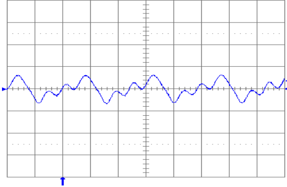
Fig. 2.0V.7: Output voltage ripple (20 mV/div.) at full rated load current into a resistive load with C_o = 10\ \mu\text{F} tantalum + 1\ \mu\text{F} ceramic and V_{in} = 48\ \text{V} . Time scale: 1\ \mu\text{s}/\text{div} .
