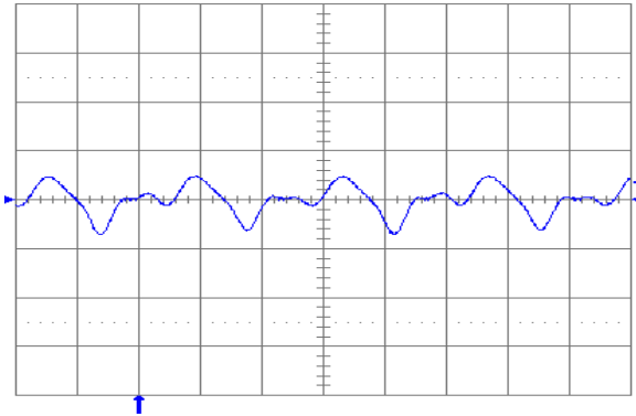
Fig. 1.2V.7: Output voltage ripple (20 mV/div.) at full rated load current into a resistive load with C_o = 10\ \mu\text{F} tantalum + 1\ \mu\text{F} ceramic and V_{in} = 48\ \text{V} . Time scale: 1\ \mu\text{s}/\text{div} .
