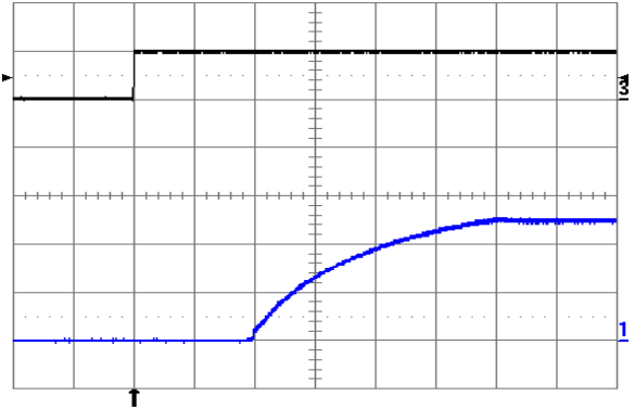
Fig. 2.5V.4: Turn-on transient at full rated load current (resistive) plus 20,000 \mu\text{F} at V_{in} = 48\text{ V} , triggered via ON/OFF pin. Top trace: ON/OFF signal (5 V/div.). Bottom trace: output voltage (1 V/div.). Time scale: 2 ms/div.
