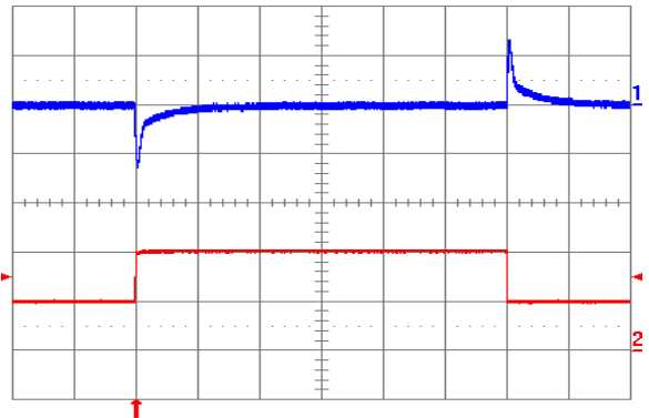
Fig. 2.5V.6: Output voltage response to load current step-change (5 A – 10 A – 5 A) at V_{in} = 48\text{ V} . Top trace: output voltage (100 mV/div.). Bottom trace: load current (5 A/div.). Current slew rate: 5 A/ \mu\text{s} . C_o = 450\ \mu\text{F} tantalum + 1 \mu\text{F} ceramic. Time scale: 0.2 ms/div.
