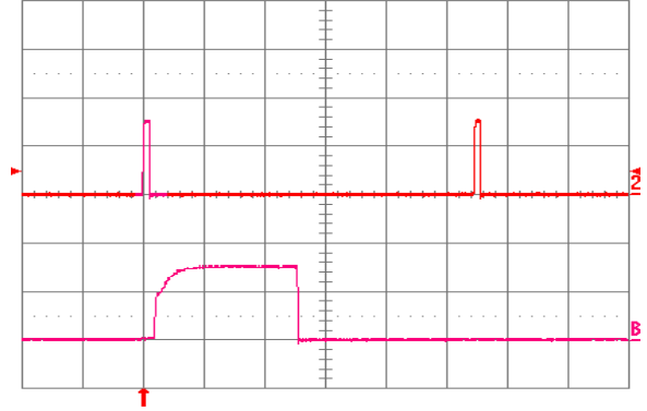
Fig. 2.0V.12: Load current (top trace, 20 A/div., 20 ms/div.) into a 10 mΩ short circuit during restart, at Vin = 48 V. Bottom trace (20 A/div., 1 ms/div.) is an expansion of the on-time portion of the top trace.
