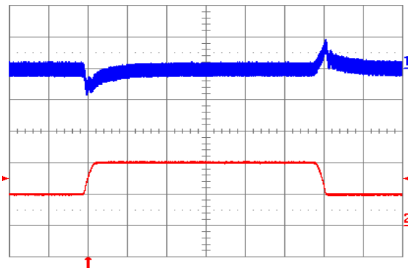
Fig. 2.5V.5: Output voltage response to load current step-change (5 A – 10 A – 5 A) at V_{in} = 48\text{ V} . Top trace: output voltage (100 mV/div.). Bottom trace: load current (5 A/div.). Current slew rate: 0.1 A/ \mu\text{s} . C_o = 1\ \mu\text{F} ceramic. Time scale: 0.2 ms/div.
