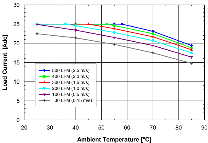
Fig. 1.5V.1: Available load current vs. ambient air temperature and airflow rates for SQM48T25015 converter with D height heat pins mounted vertically with air flowing from pin 3 to pin 1, MOSFET temperature \leq 120^\circ\text{C} , V_{in} = 48\text{ V} .
