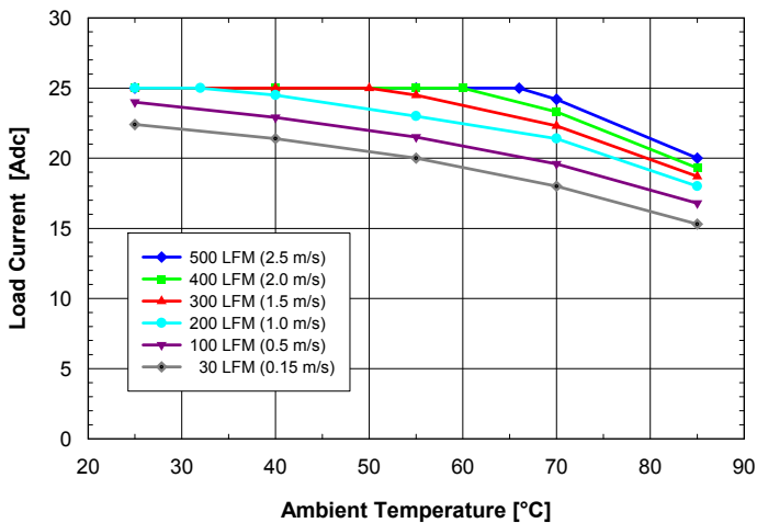
Fig. 1.2V.1: Available load current vs. ambient air temperature and airflow rates for SQM48T25012 converter with D height heat pins mounted vertically with air flowing from pin 3 to pin 1, MOSFET temperature \leq 120^\circ\text{C} , V_{in} = 48\text{ V} .
