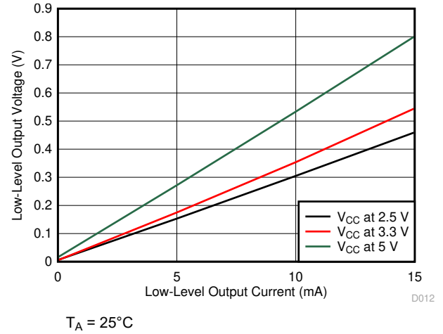
Figure 7-10. Low-Level Output Voltage vs Low-Level Output Current
