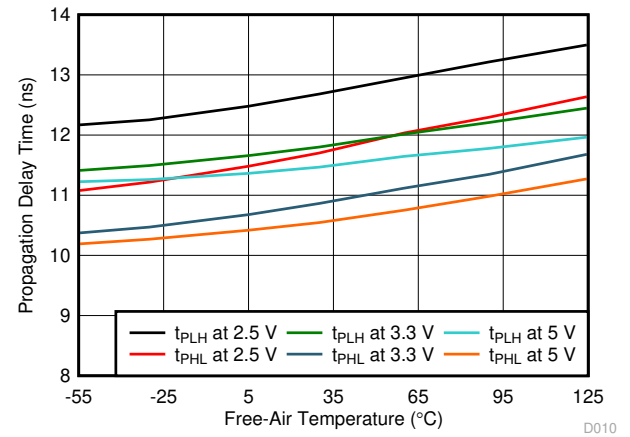
Figure 7-12. Propagation Delay Time vs Free-Air Temperature
