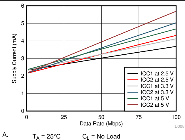
Figure 7-8. ISO7731-Q1 Supply Current vs Data Rate (With No Load)
