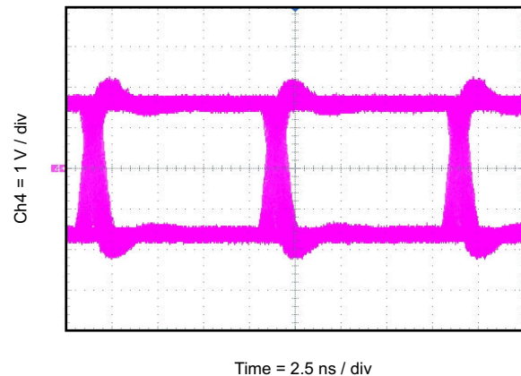
Figure 10-5. Eye Diagram at 100 Mbps PRBS 2 16 – 1, 3.3 V and 25°C
