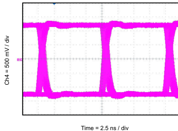
Figure 10-6. Eye Diagram at 100 Mbps PRBS 2 16 – 1, 2.5 V and 25°C
