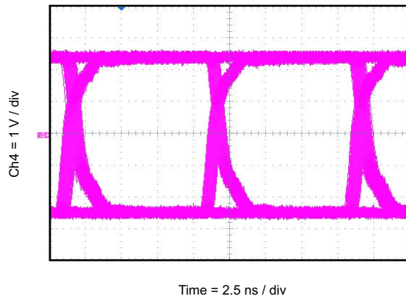
Figure 10-4. Eye Diagram at 100 Mbps PRBS 2 16 – 1, 5 V and 25°C
