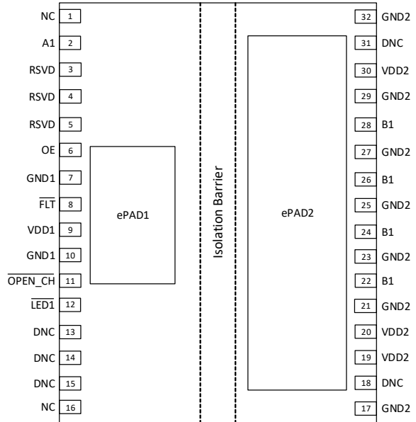
Si83411xBA-IF
