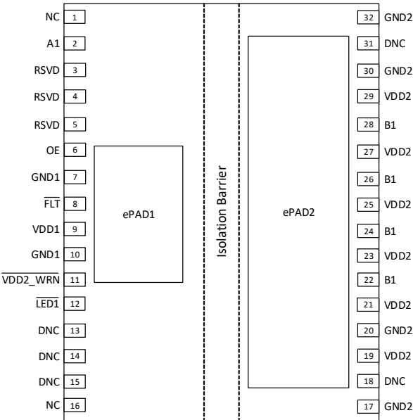
Si83401xAA-IF
