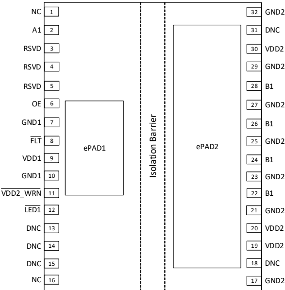
Si83411xAA-IF
