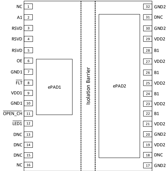
Si83401xBA-IF
