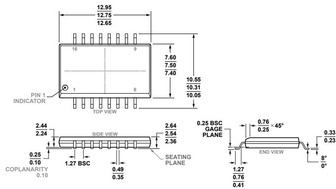
Figure 25. 16-Lead Standard Small Outline Package, with Increased Creepage [SOIC_IC] Wide Body (RI-16-2) Dimensions shown in millimeters
