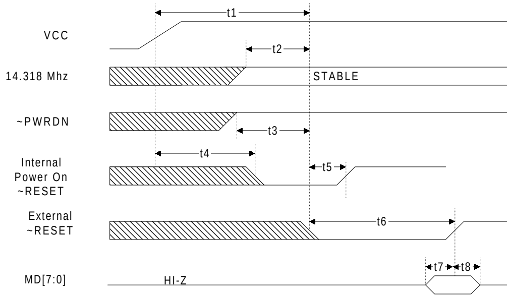
Figure 46: Power-on Reset and Reset Configuration Timing
