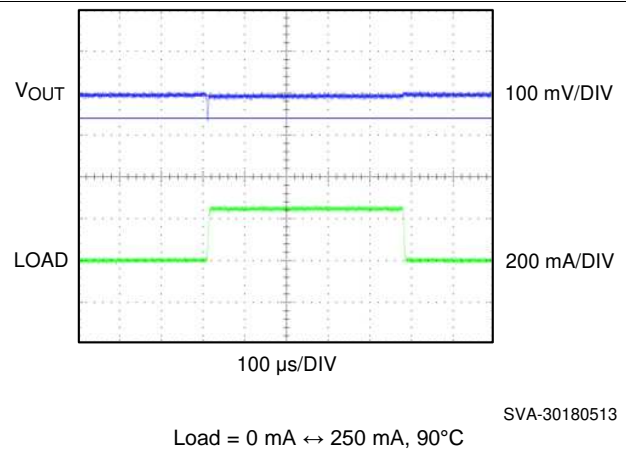
Figure 12. Load Transient
