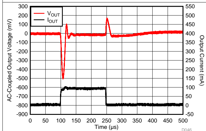
Output current slew rate = 100 mA/µs
