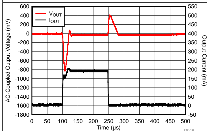
Output current slew rate = 200 mA/µs
