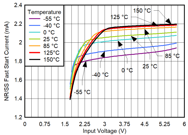
Figure 8-12. I_{FAST\_SS} Reference vs Input Voltage and Temperature for V_{OUT} = 3.3\text{ V}
