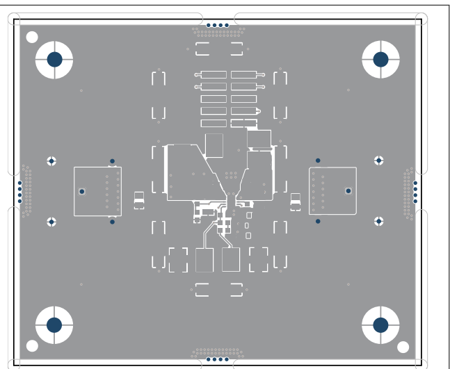
Figure 8-20. Top Layer Routing
