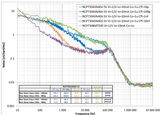
Figure 51. Noise – ADJ-set-5.0 V with Different C_{FF} and FIX – 5.0 V
