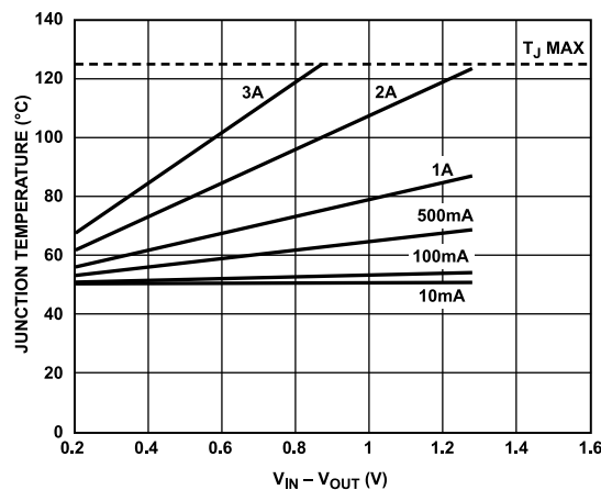
Figure 42. 500 mm 2 of PCB Copper, T B = 50°C
