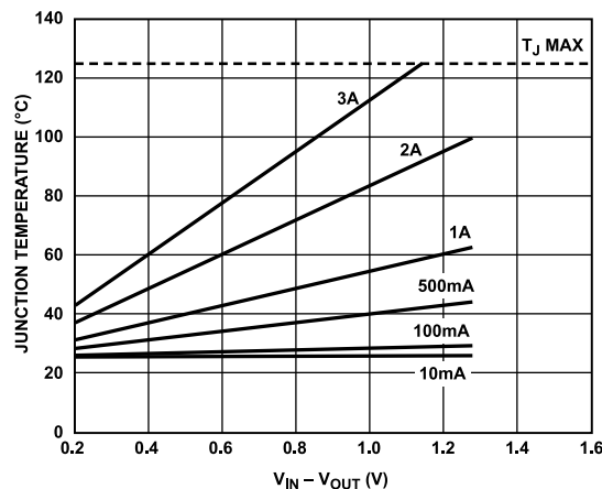
Figure 41. 500 mm 2 of PCB Copper, T B = 25°C
