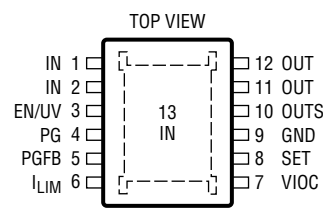
MSE PACKAGE 12-LEAD PLASTIC MSOP T JMAX = 150°C, θ JA = 33°C/W, θ JC = 8°C/W EXPOSED PAD (PIN 13) IS IN, MUST BE SOLDERED TO PCB
