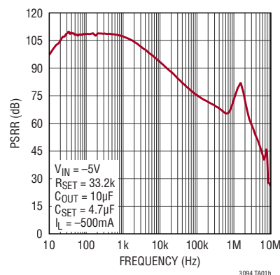
Power Supply Ripple Rejection
