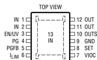
MSE PACKAGE 12-LEAD PLASTIC MSOP T_{JMAX} = 150^{\circ}\text{C} , \theta_{JA} = 33^{\circ}\text{C/W} , \theta_{JC} = 8^{\circ}\text{C/W} EXPOSED PAD (PIN 13) IS IN, MUST BE SOLDERED TO PCB
