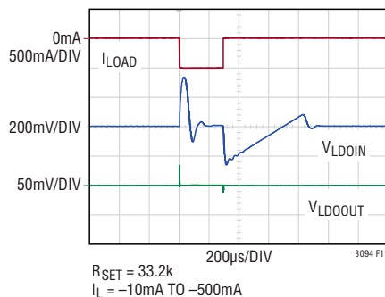
Figure 11. Load Step Response Using the VIOC Buffer
