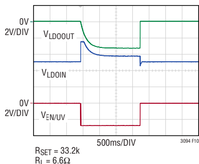
Figure 10. LT3094 EN/UV Pulse
