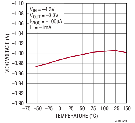
VIOC Voltage
