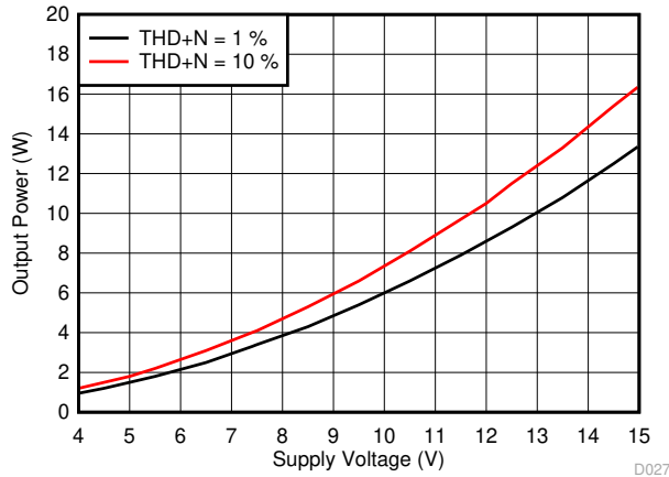
Figure 6-28. Output Power vs Supply Voltage, 8 Ω
