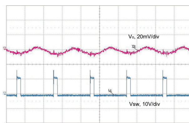
Fig. 55 - Output Ripple, 6 A, t = 1\text{ }\mu\text{s}/\text{div} Forced Continuous Conduction Mode
