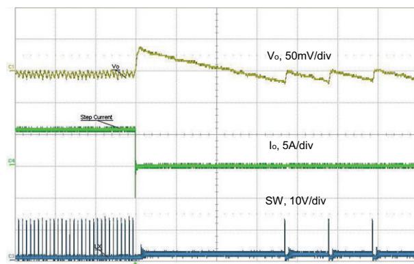
Fig. 53 - Load Release, 6 A to 0.1 A, 1 A/ \mu\text{s} , t = 20\text{ }\mu\text{s}/\text{div} Skip Mode Enabled
