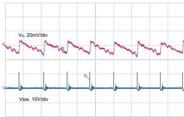
Fig. 52 - Output Ripple, 0.1 A, t = 20\text{ }\mu\text{s}/\text{div} Skip Mode Enabled
