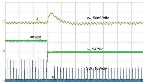
Fig. 54 - Load Release, 6 A to 0.1 A, 1 A/ \mu\text{s} , t = 10\text{ }\mu\text{s}/\text{div} Forced Continuous Conduction Mode
