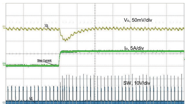
Fig. 51 - Load Step, 0.1 A to 6 A, 1 A/ \mu\text{s} , t = 10\text{ }\mu\text{s}/\text{div} Forced Continuous Conduction Mode
