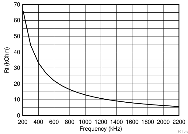
Figure 9-4. Setting Clock Frequency
