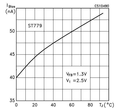
Figure 12 : FB Pin Bias Current vs Temperature
