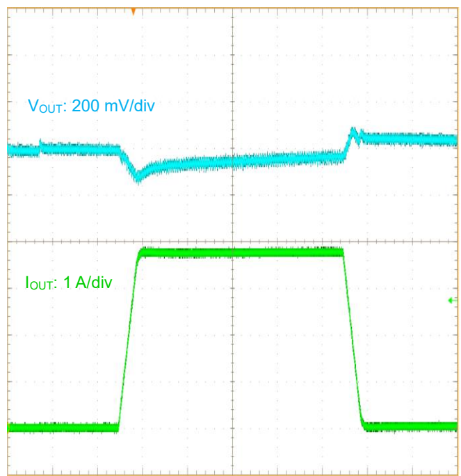
Figure 42. Load Transient Response ( I_{OUT} = 0\text{ A} - 3.75\text{ A} )
