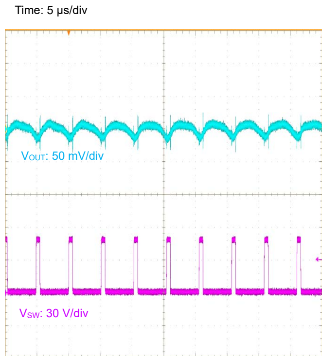
Figure 40. V_{OUT} Ripple ( I_{OUT} = 5.0\text{ A} )
