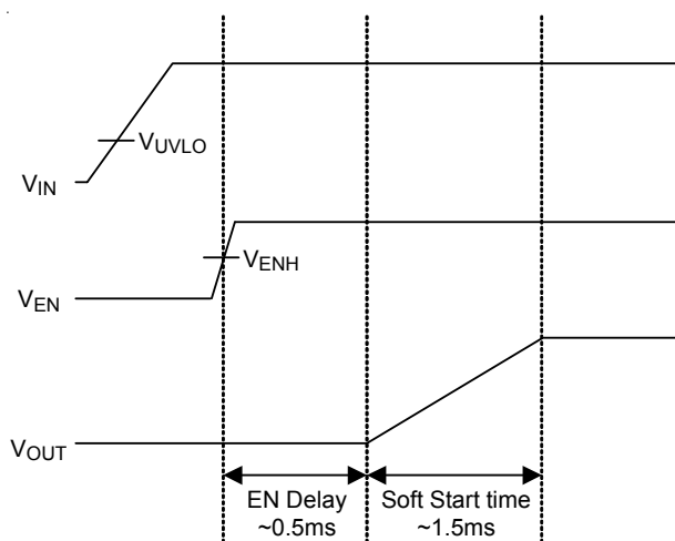
Figure 2. Power Up Sequence
