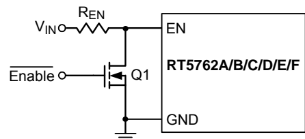
Figure 7. Logic Control for the EN Pin
