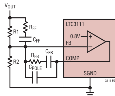
Figure 7: Error Amplifier with Type III Compensation
