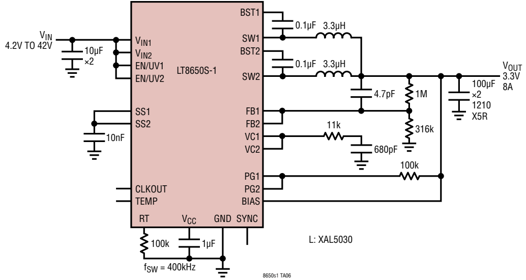
Two Phase, 3.3V, 8A, 400kHz Step-Down Converter
