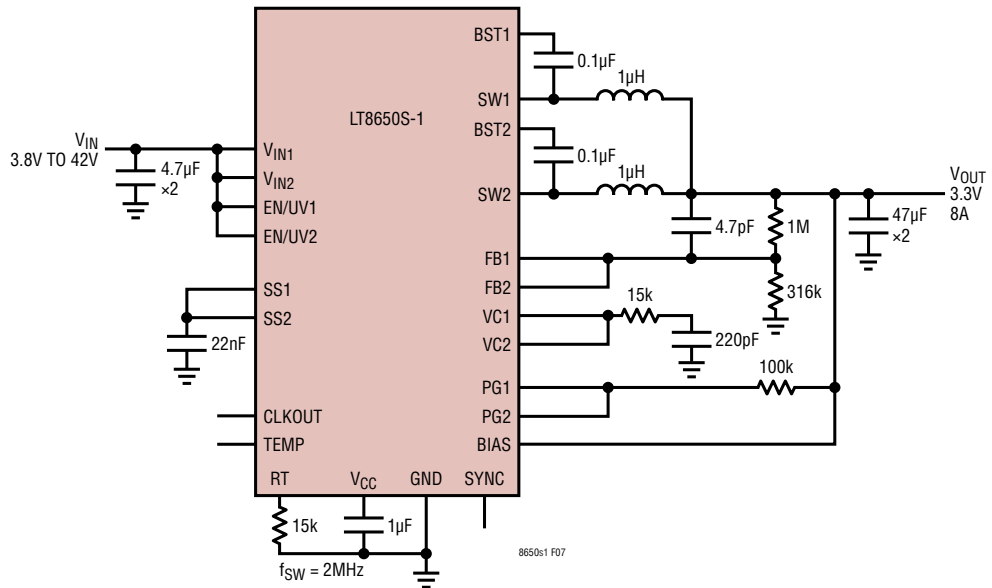
Figure 7 Two-Phase Application
