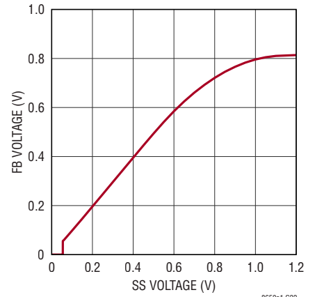
Soft-Start Tracking
