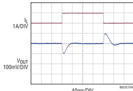
0A TO 1A TRANSIENT 3.3V OUT , D0 = D1 = 0V C OUT = 100µF FCM, f SW = 2MHz (R T = 15kΩ)
