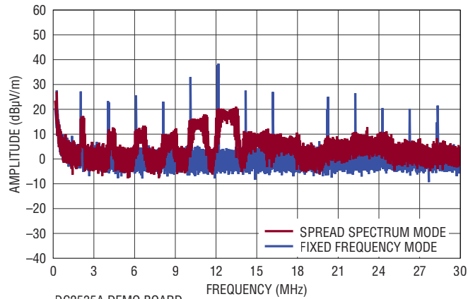
DC2535A DEMO BOARD (WITH EMI FILTER INSTALLED) 8653S G42 14V INPUT TO 5V OUTPUT1 AT 2A AND 3.3V OUTPUT2 AT 2A, f_{SW} = 2\text{MHz}
