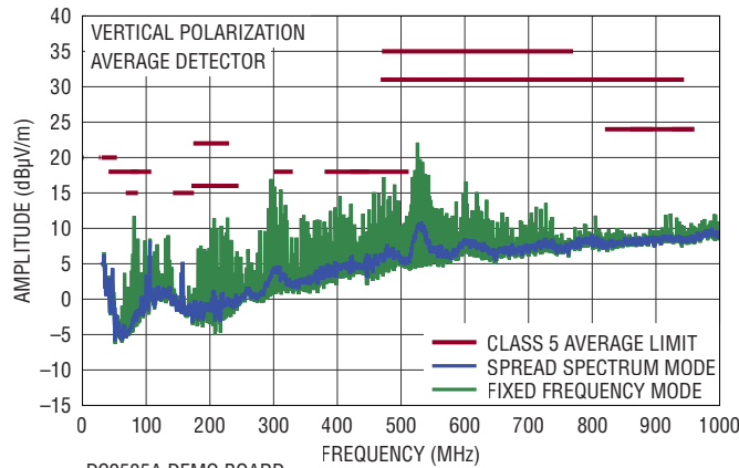
DC2535A DEMO BOARD (WITH EMI FILTER INSTALLED) 8653S G44 14V INPUT TO 5V OUTPUT1 AT 2A AND 3.3V OUTPUT2 AT 2A, f_{SW} = 2\text{MHz}
