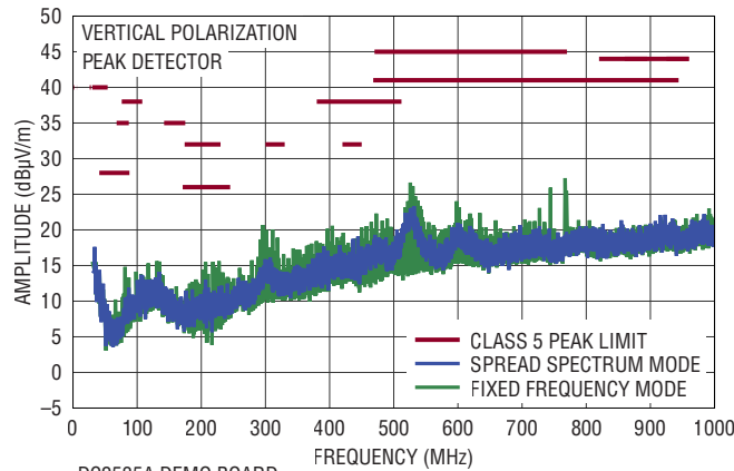
DC2535A DEMO BOARD (WITH EMI FILTER INSTALLED) 8653S G43 14V INPUT TO 5V OUTPUT1 AT 2A AND 3.3V OUTPUT2 AT 2A, f_{SW} = 2\text{MHz}
