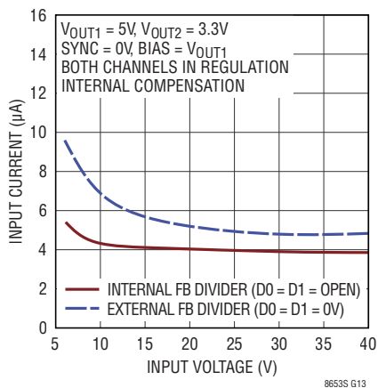
No Load Supply Current with Internal Compensation
