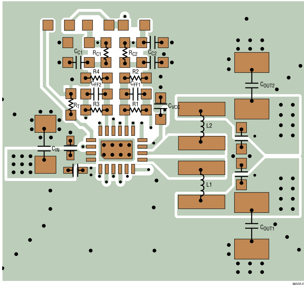
Figure 9. Recommended Layout
