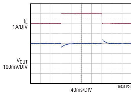
0A TO 1A TRANSIENT 3.3V OUT , D0 = D1 = 0V C OUT = 100µF FCM, f SW = 2MHz (R T = 15kΩ) C C = 470pF, R C = 34.8kΩ
