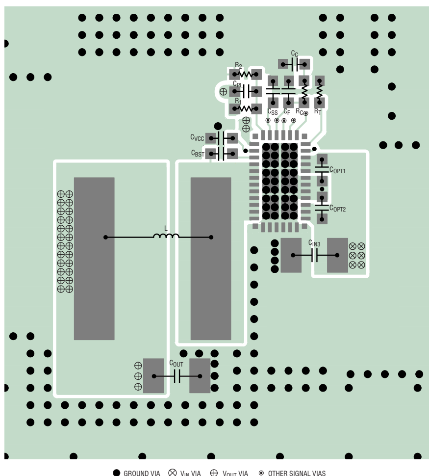
Figure 1. Recommended PCB Layout
