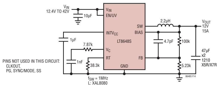
Figure 14. 1MHz 12V, 15A Step-Down Converter
