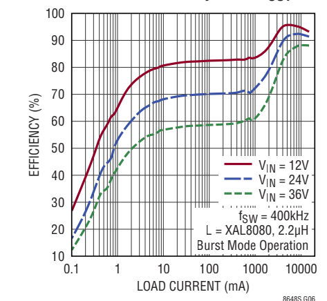
Low Load Efficiency at 3.3V OUT
