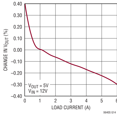
LT8643S Load Regulation
