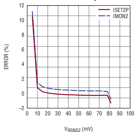
ISET2P and IMON2 Measurement Accuracy
