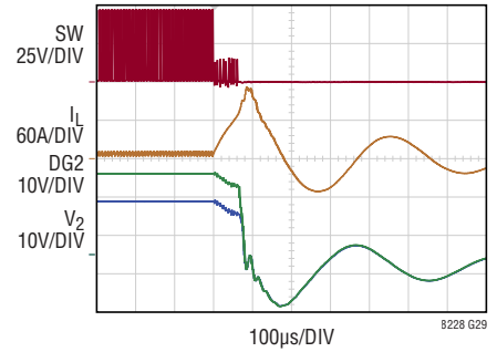
BG MOSFET Short in Regulation (Boost)
