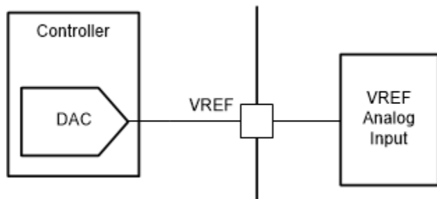
Figure 7-4. Controlling VREF with a DAC Resource
