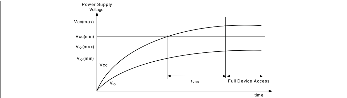
Figure 9 Power-up
